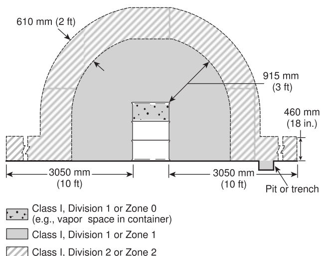
FIGURE 6.5.5.2 Electrical Area Classification for Class I Liquid Operations Around Open Containers, Supply Containers, Waste Containers, Spray Gun Cleaners, and Solvent Distillation Units.
