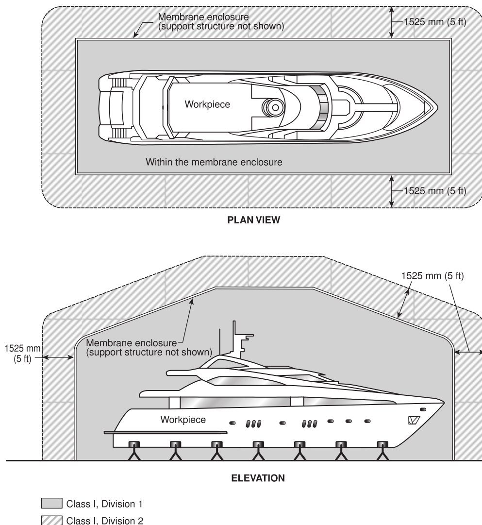
▲ FIGURE 18.6.1.2 Electrical Classifications for Outdoor Membrane Enclosures.
