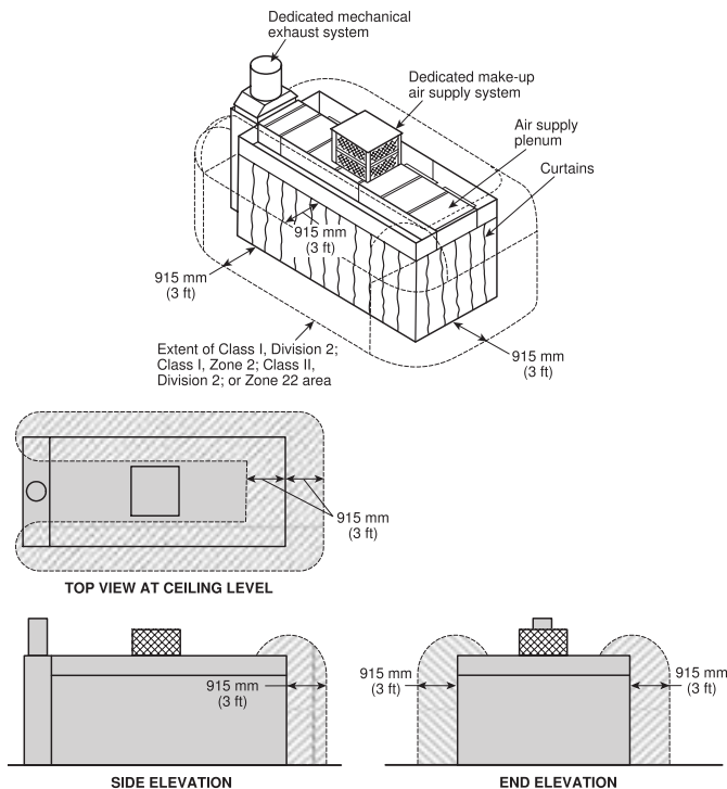
▲ FIGURE 14.3.6.1 Class I, Division 2; Zone 2; Class II, Division 2; or Zone 22 Locations Adjacent to a Limited Finishing Workstation.
