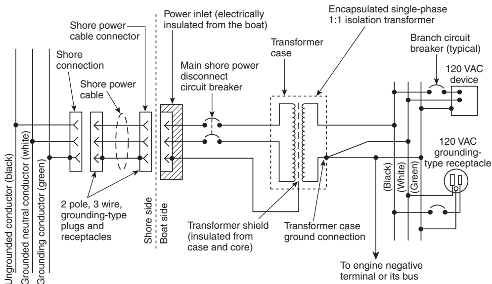
FIGURE 10.18.4.3(f) Single-Phase 120-Volt Isolation Transformer System with Boat-Grounded Secondary, Shore-Grounded Transformer Shield, and Boat-Grounded Transformer Metal Case.
