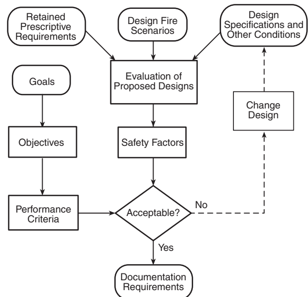
FIGURE A.5.1.1 Performance-Based Life Safety Code Compliance Process.
