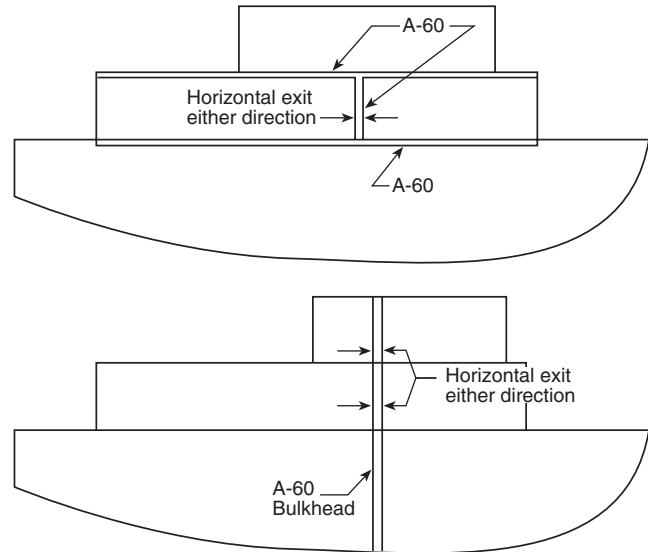
FIGURE A.3.3.22.1 Horizontal Exit.
