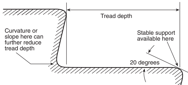
FIGURE A.6.2.2.2.3(d) Tread measurement with stable support at leading edge.
