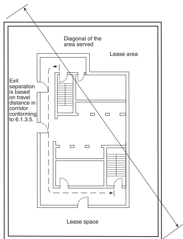
FIGURE A.6.5.1.5(d) Exit separation measured along corridor path.
