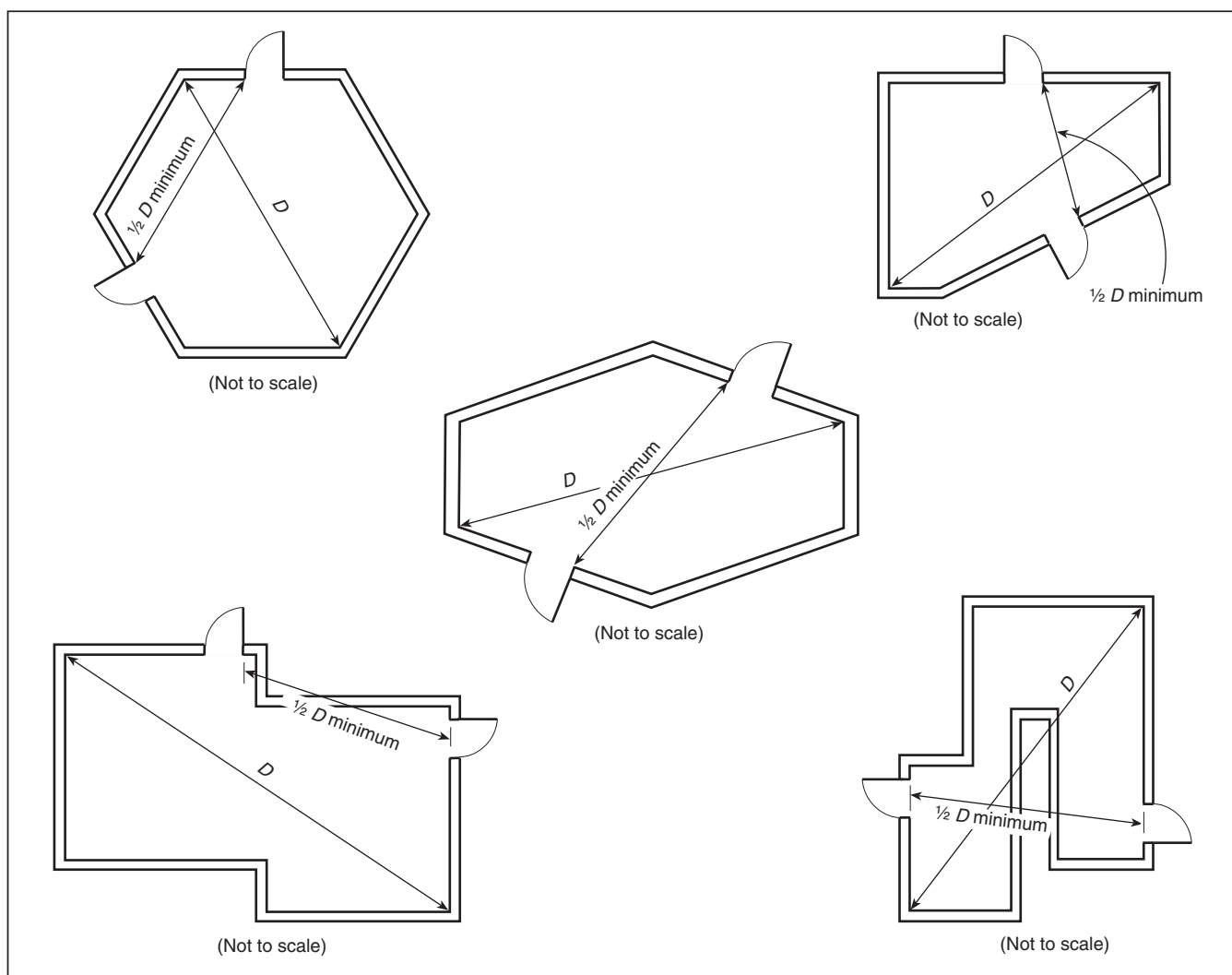
FIGURE A.6.5.1.5(e) Diagonal measurement for unusually shaped areas.
