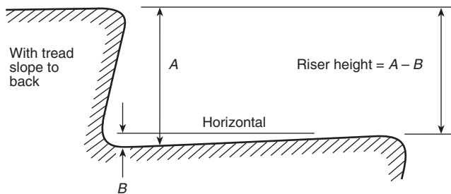
FIGURE A.6.2.2.2.3(b) Riser measurement with tread slope to back.
