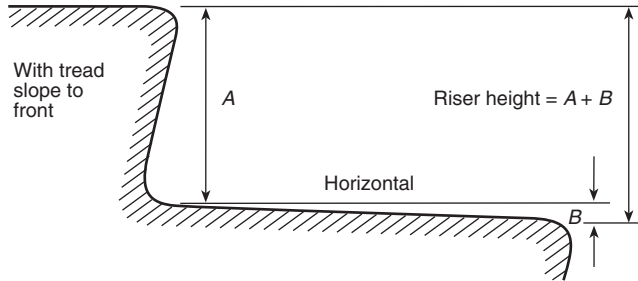
FIGURE A.6.2.2.2.3(a) Riser measurement with tread slope to front.
