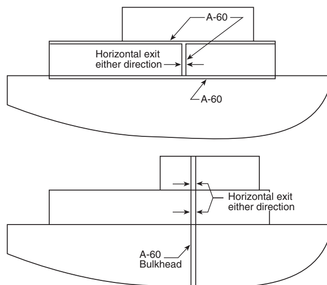
FIGURE A.3.3.22.1 Horizontal exit. A-60 is generally required for horizontal exits, but can be modified as allowed by Chapters 18 through 20.
