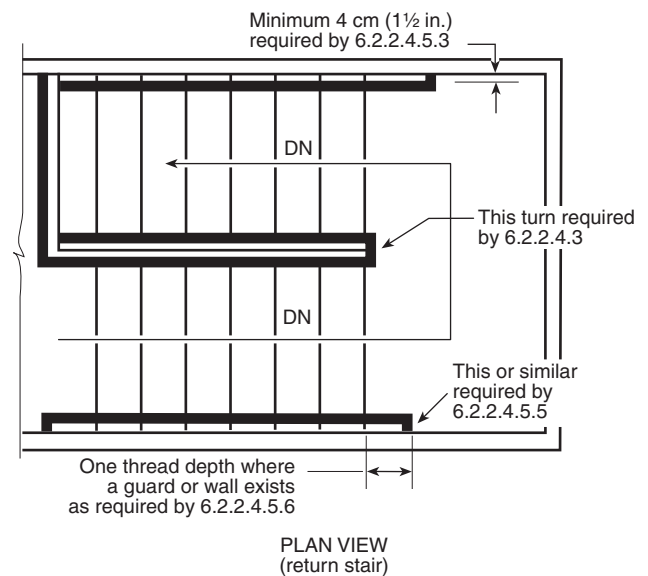
FIGURE A.6.2.2.4.5 Handrail details.
