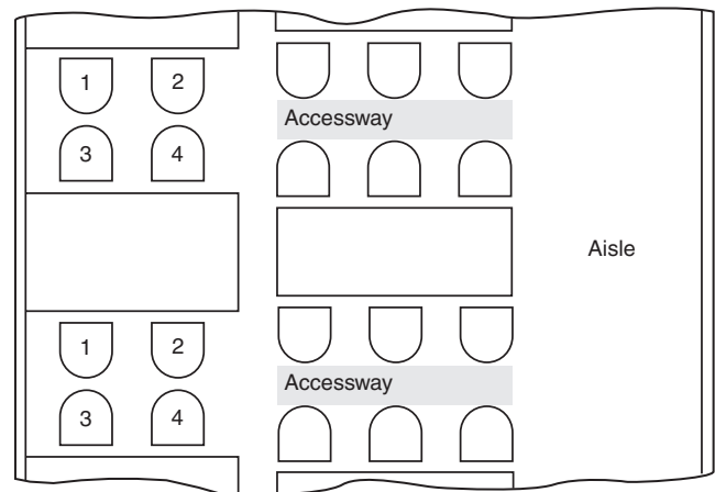
FIGURE A.6.2.11(a) Aisle accessways between rows of theater style seating.
