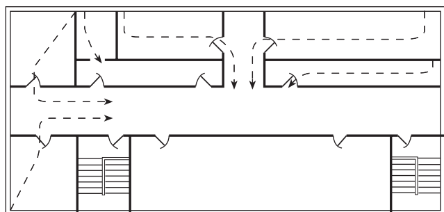
FIGURE A.3.3.11 Common paths of travel. The portion of the exit access travel for which an occupant is steered in one direction only, without the option of traveling in another independent direction toward an exit, is a common path of travel. Common paths of travel are illustrated by the dashed lines.
