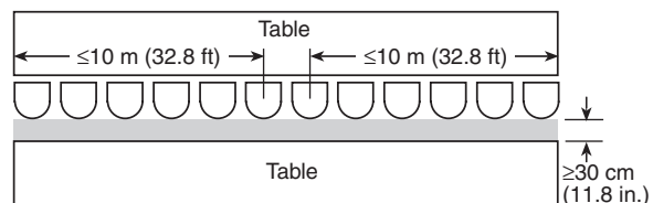
FIGURE A.6.2.11(b) Aisle accessway width \geq 30 cm (11.8 in.).
