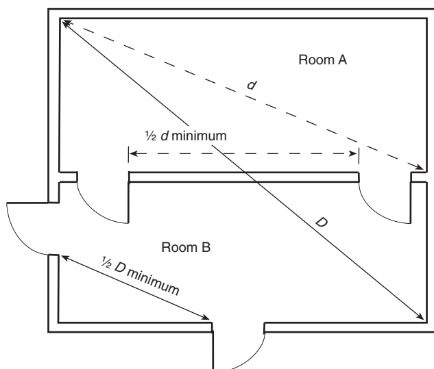
FIGURE A.6.5.1.5(b) Communicating openings, whether protected or not, between the stair enclosures.
