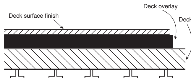
FIGURE A.7.3.4 Deck overlay details.
