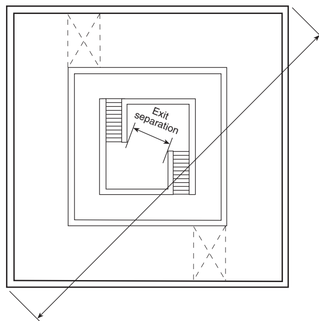
FIGURE A.6.5.1.5(c) Exit separation and diagonal measurement of area served.
