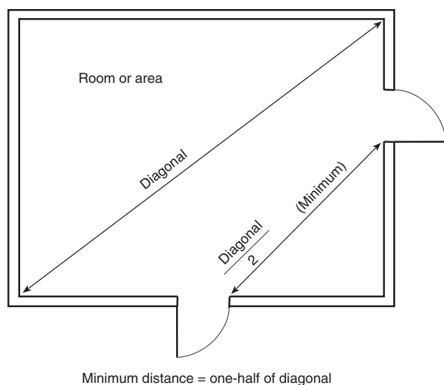
FIGURE A.6.5.1.5(a) Remoteness and half-diagonal rule.
