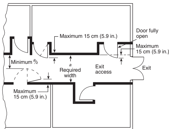
FIGURE A.6.2.1.4.3 Door swing into a corridor.
