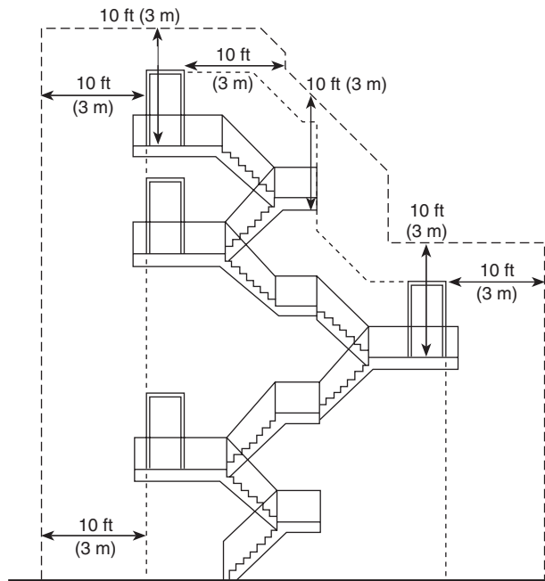
FIGURE A.6.2.2.6.2 Protection of outside stairs. Fire resistance rating for the bulkhead of the 10-ft (3-m) extension is a minimum of 1 hour.
