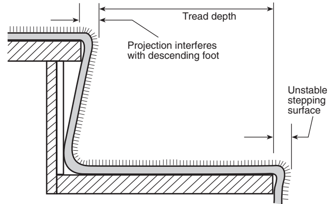
FIGURE A.6.2.2.2.3(e) Tread measurement with unstable stepping surface at leading edge.
