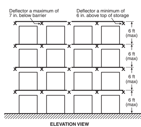
FIGURE 16.6.2.1(a) Single-Row Rack Sprinkler Layout for Design Scheme “B” — Sprinklers in Center of Rack.
