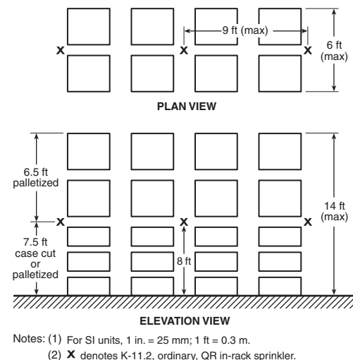
FIGURE 16.6.4(a) Double-Row Rack Sprinkler Layout 7.
