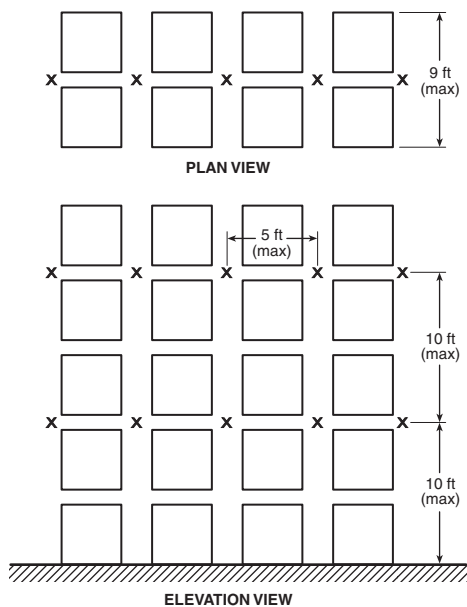
FIGURE 16.6.4(e) Double-Row Rack Sprinkler Layout 9 — Option #2.
