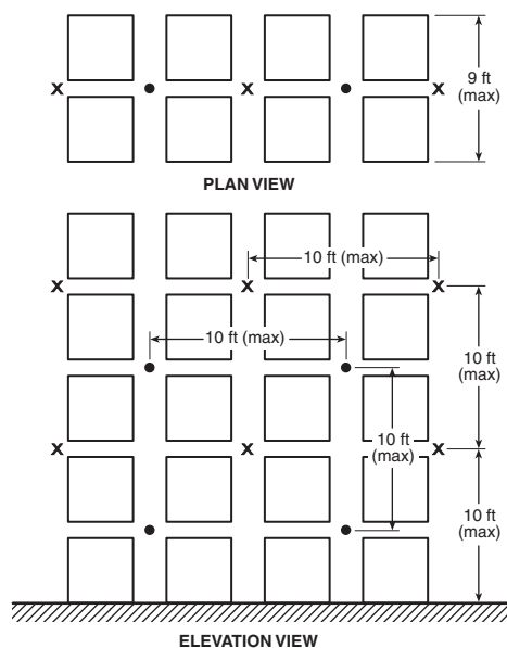
FIGURE 16.6.4(d) Double-Row Rack Sprinkler Layout 9 — Option #1.
