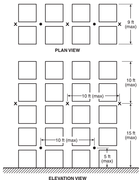
FIGURE 16.6.4(b) Double-Row Rack Sprinkler Layout 8 — Option #1.
