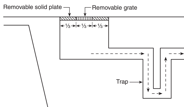
FIGURE A.16.8.2(c) Details of Drainage Trench Design.
