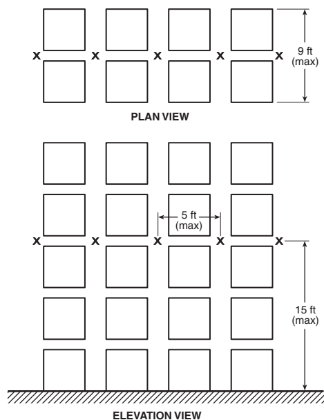
FIGURE 16.6.4(c) Double-Row Rack Sprinkler Layout 8 — Option #2.
