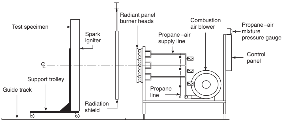
FIGURE 5.1.5(b) Side elevation of the test apparatus.
