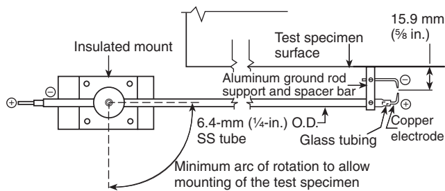
FIGURE 5.4.2.1(a) Plan view of the spark igniter.
