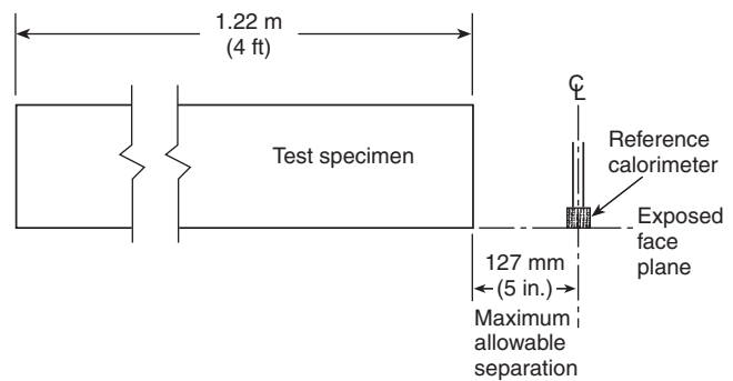
FIGURE 6.1.1 Plan view of reference calorimeter location.
