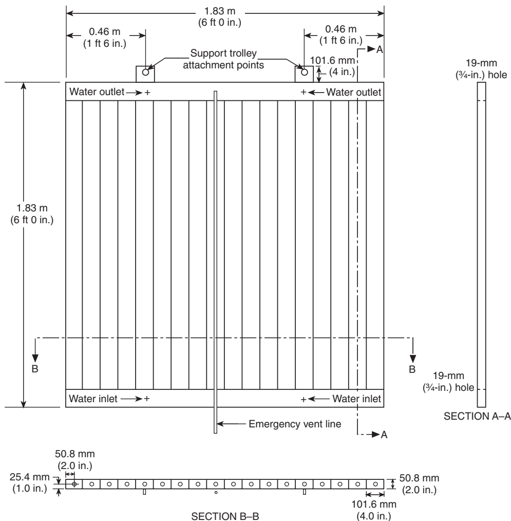
FIGURE A.5.3.1 Radiation shield.
