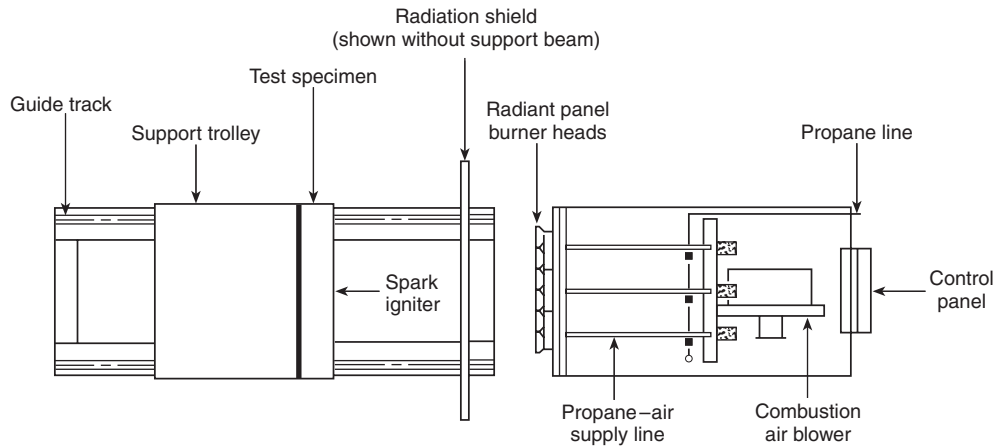
FIGURE 5.1.5(a) Plan view of the test apparatus.
