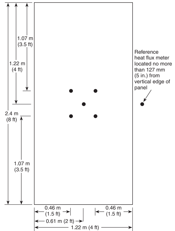
FIGURE 6.1.2 Calibration panel heat flux meter locations.
