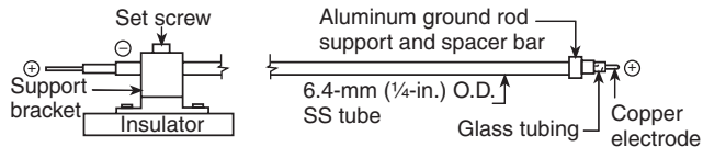
FIGURE 5.4.2.1(b) Side elevation of the spark igniter.
