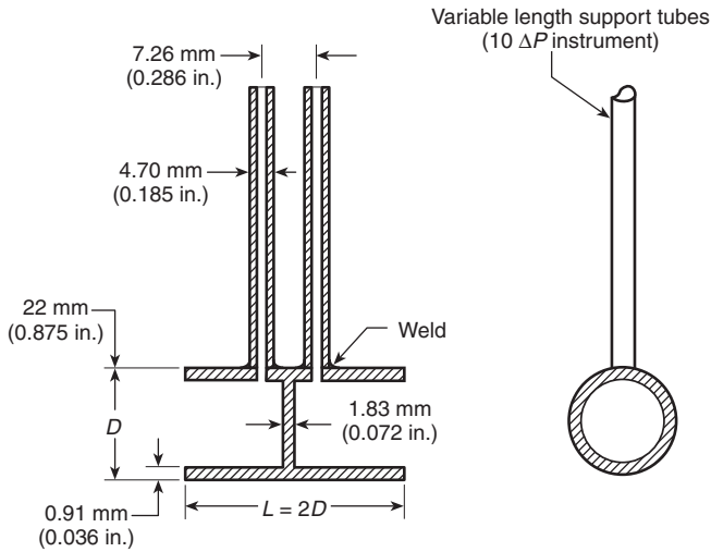
FIGURE 7.3.2.1 Bidirectional Probe.
