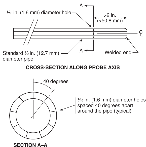
FIGURE 4.3.1.2(b) Pressure Probe.
