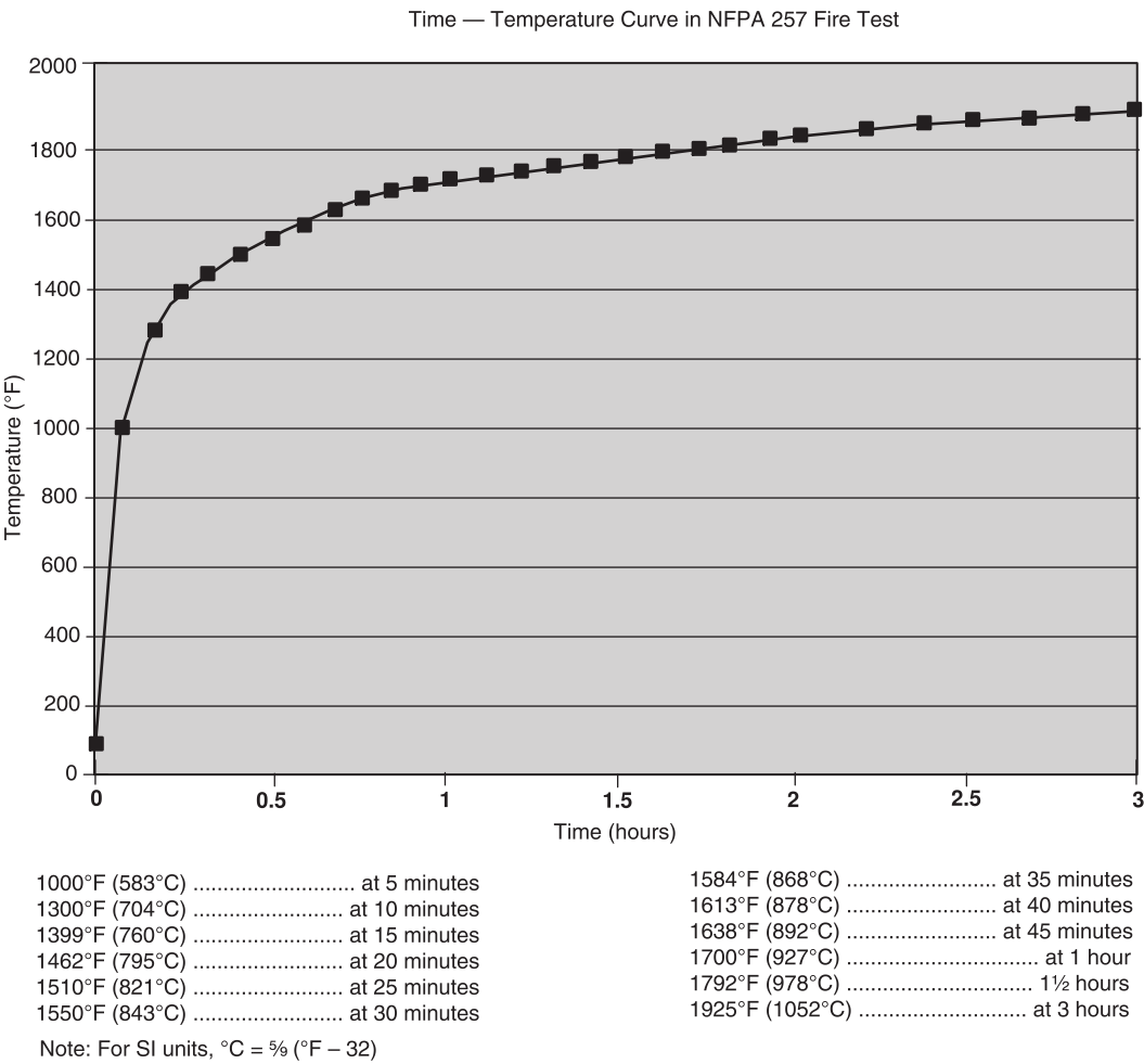
FIGURE 4.1.1 Temperature–Time Curve.
