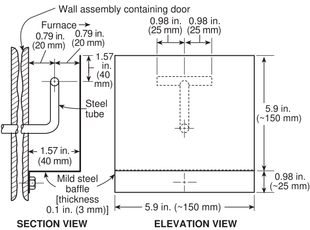
FIGURE 4.3.1.2(a) Static Pressure-Measuring Device Dimensions.
