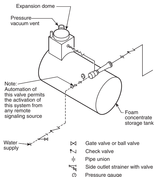
FIGURE A.3.3.33.3 Line Proportioner.
