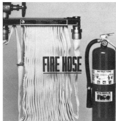
FIGURE A.3.3.19.4 Semiautomatic Hose Rack Assembly.
