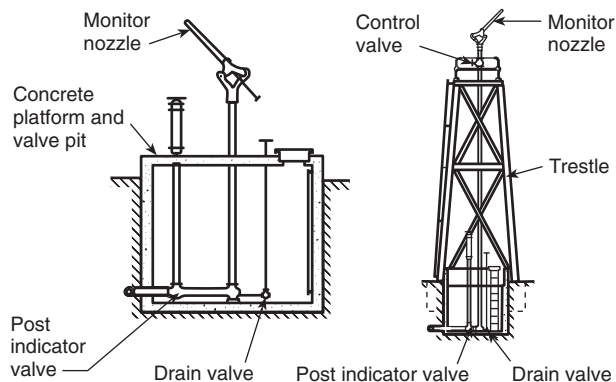
FIGURE A.3.3.27.1(a) Standard Monitor Nozzles; Gear Control Nozzles Also Are Permitted.
