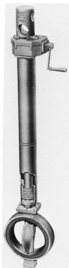
FIGURE A.13.1(b) Butterfly Post Indicator Valve. (Courtesy of Henry Pratt Co.)
