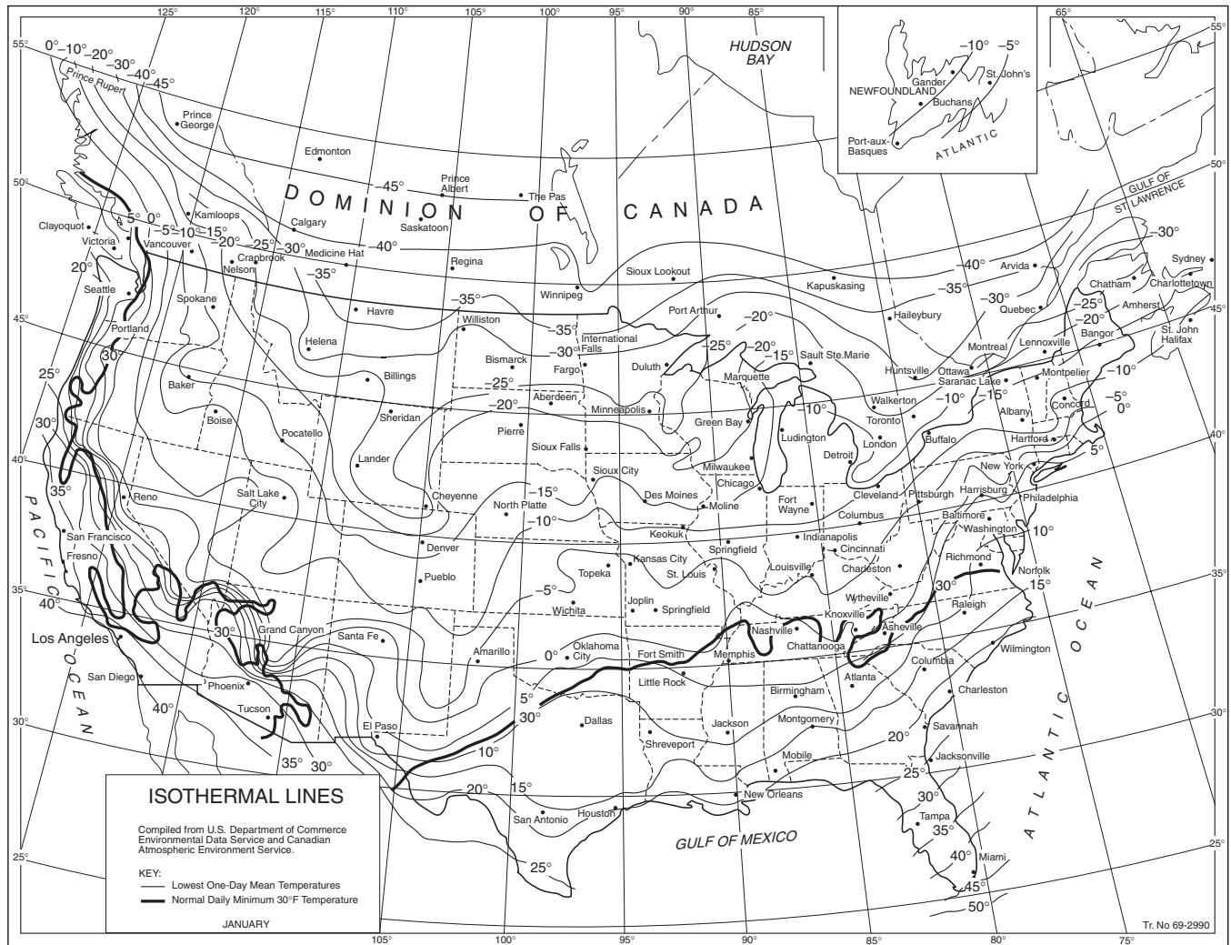
FIGURE A.5.3.4 Isothermal Lines — Lowest One-Day Mean Temperature ( ^{\circ}\text{F} ). [24:Figure A.10.5.1]
