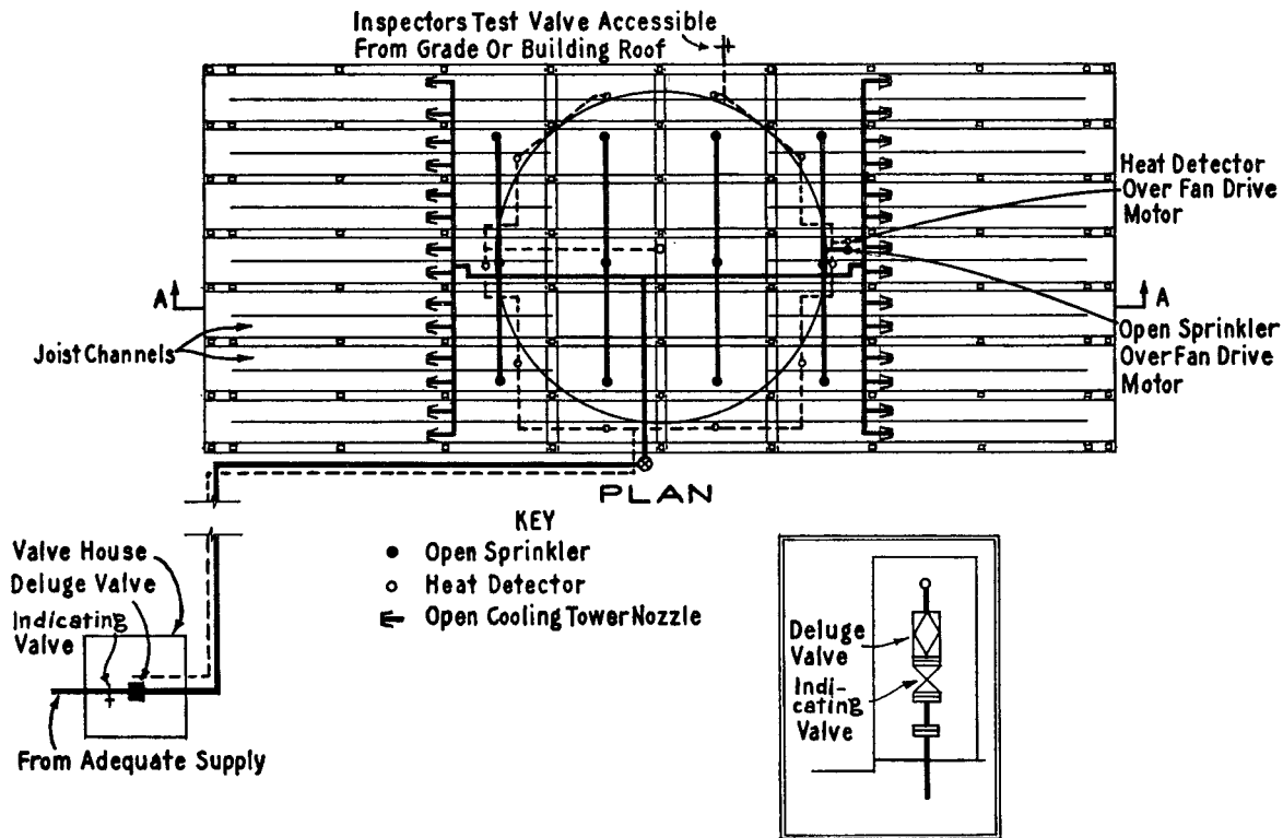
Figure B-9 Typical deluge fire protection arrangement for crossflow towers.
