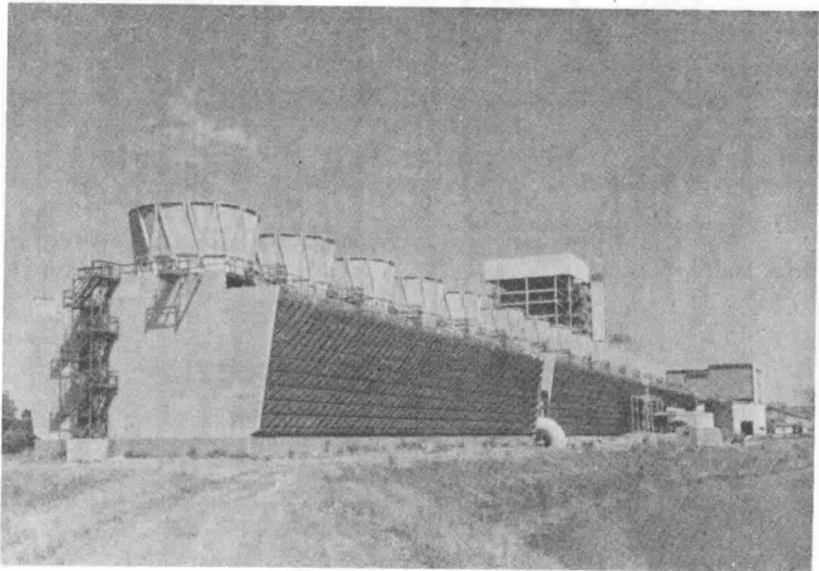
Figure B-4 Typical induced draft crossflow water-cooling tower.
