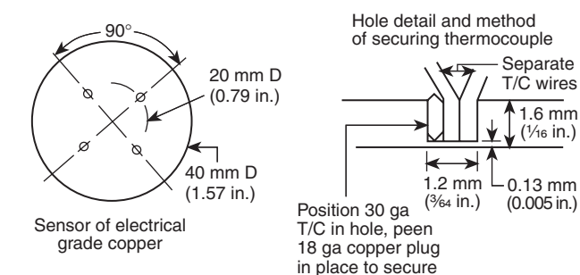
Details of calorimeter construction
