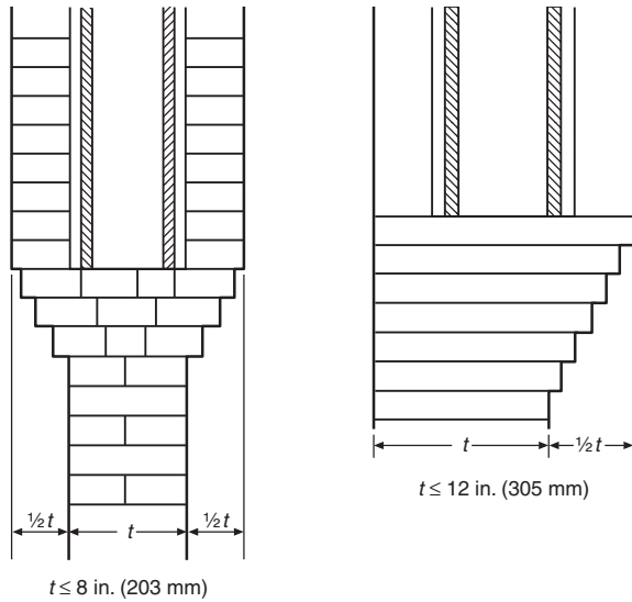
FIGURE 7.1.2(a) Corbels for Supporting Chimneys.
