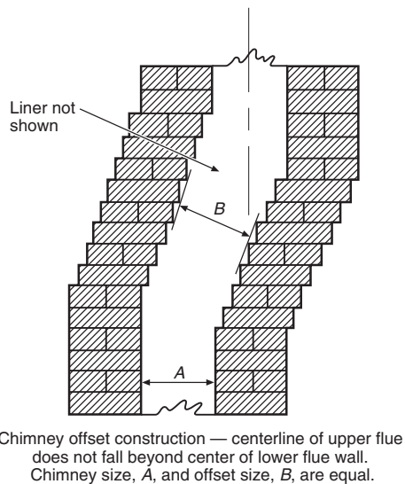
FIGURE 7.1.2(b) Corbels to Change Chimney Direction.
