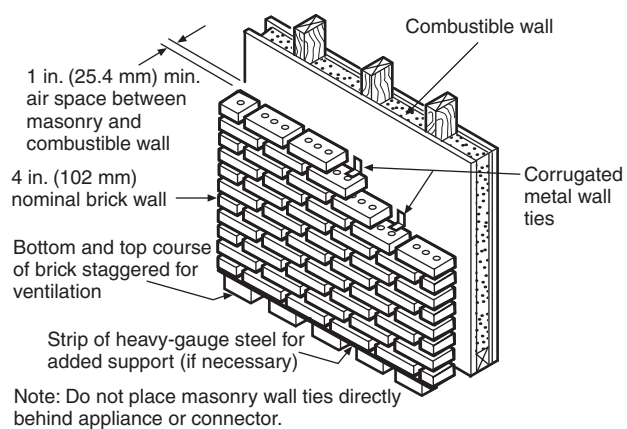
FIGURE 12.6.2.1(c) Masonry Clearance Reduction System.
