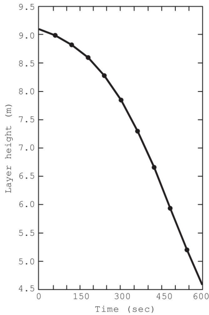
Δ FIGURE D.10(b) Layer Height.
