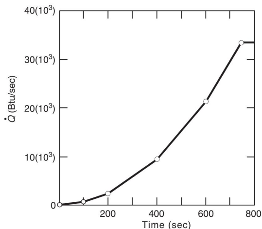
Δ FIGURE C.3(b) Energy Release Rate vs. Time for the Fire of the Default Simulation.
