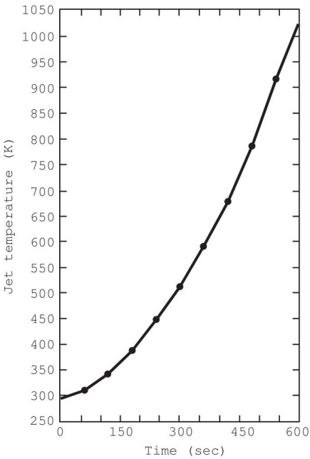
Δ FIGURE D.10(h) Jet Temperature.
