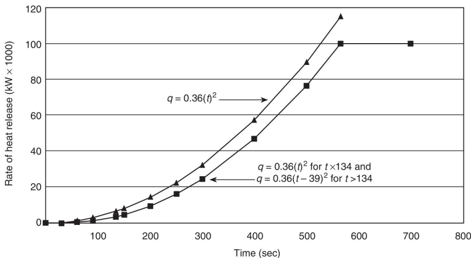
Δ FIGURE D.3 Fire Output.
