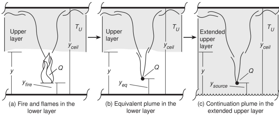
FIGURE B.4.4.1 Fire and Equivalent Source.
