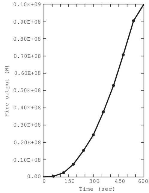
Δ FIGURE D.10(c) Fire Output.
