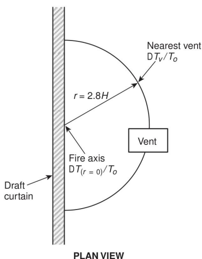
FIGURE A.5.4.3 Vent Spacing near a Draft Curtain, When r = 2.8H , (\Delta T_v/T_0) = 0.5 ( \Delta T(r=0)/T_0 ) (plan view).
