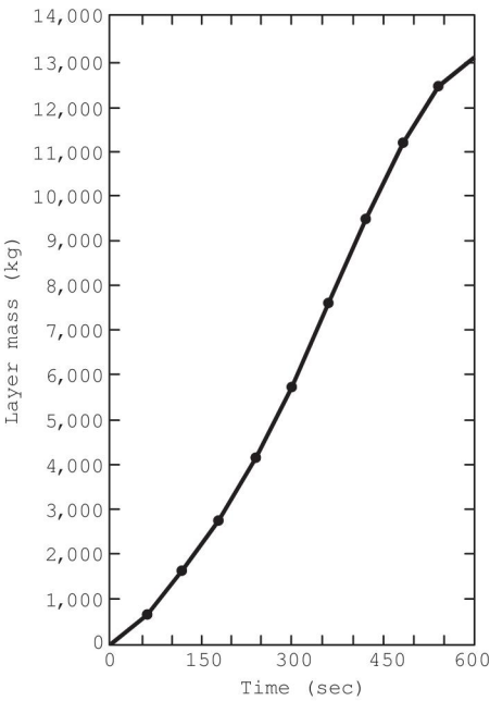
Δ FIGURE D.10(e) Layer Mass.
