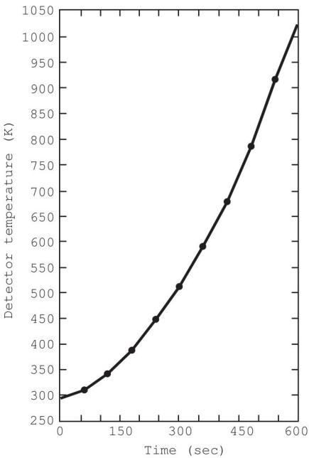
Δ FIGURE D.10(g) Detector Temperature.
