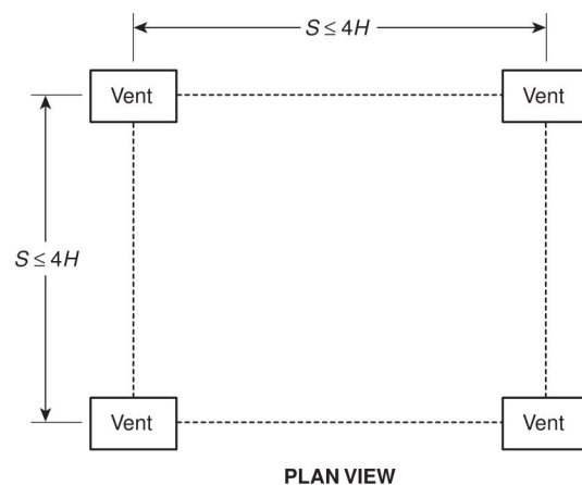
Δ FIGURE 5.4.2(a) Vent Spacing in Rectangular Matrix (plan view).
