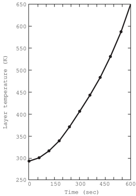
Δ FIGURE D.10(a) Layer Temperature.
