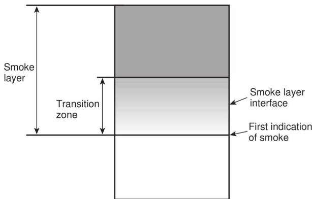
FIGURE A.3.3.3 First Indication of Smoke.
