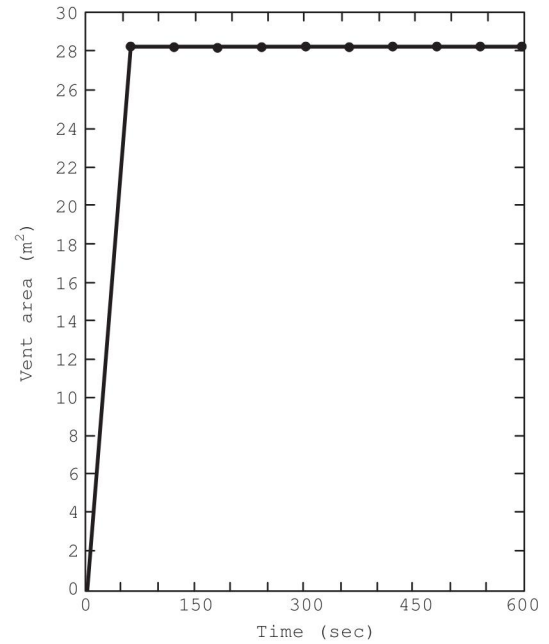
Δ FIGURE D.10(d) Vent Area.
