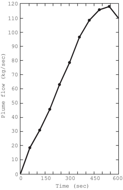
Δ FIGURE D.10(f) Plume Flow.
