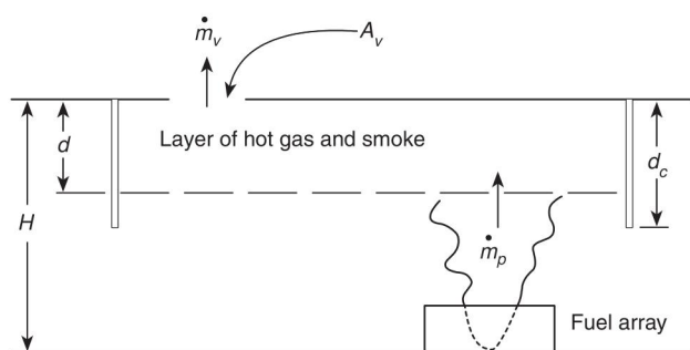
FIGURE 9.2.2.1 Schematic of Venting System.
