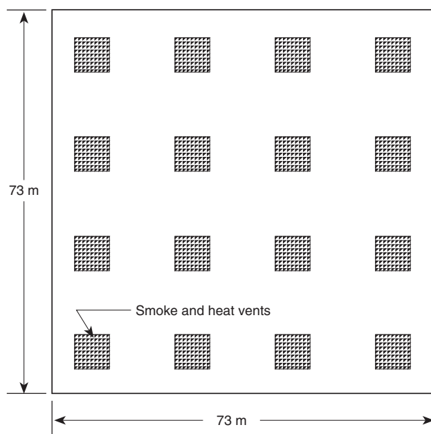
FIGURE D.2.3 Vent Plan View.
