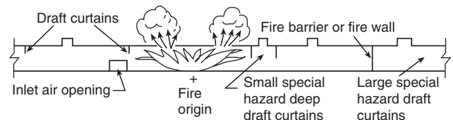
FIGURE A.1.1.1(a) Behavior of Combustion Products Under Vented and Curtained Roof.
