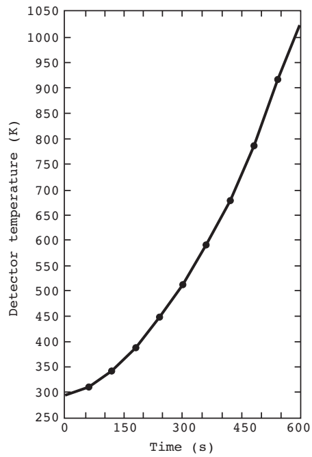
FIGURE D.10(g) Detector Temperature.
