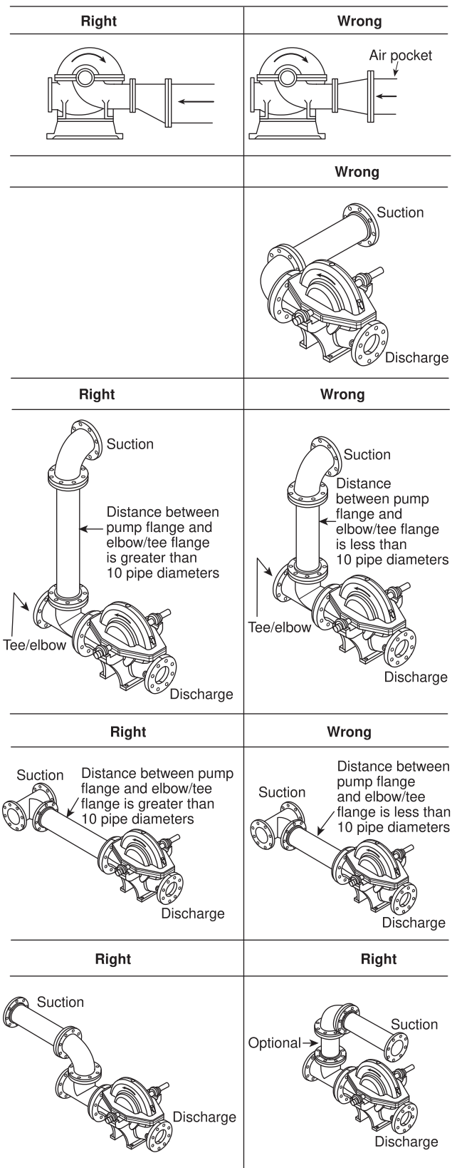
FIGURE A.4.16.6 Right and Wrong Pump Suctions.
