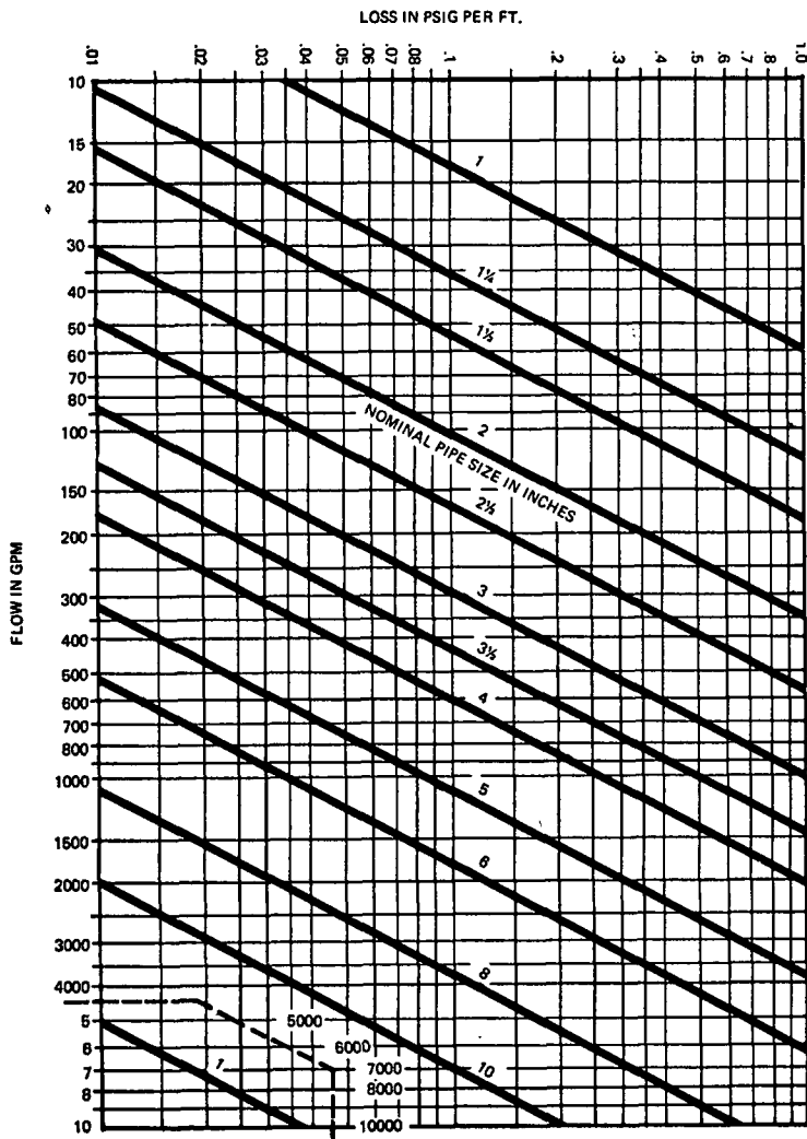
Figure A-7-2(b) Friction Loss in Schedule 40 Steel Pipe, Hazen &amp; Williams C-120.
