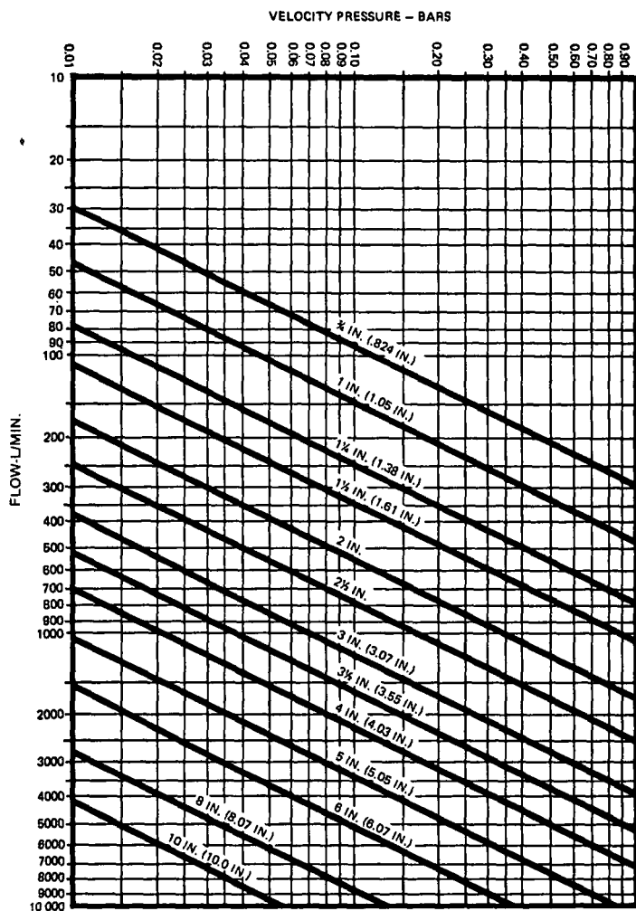
Figure A-7-2(c) Metric. Graph for the Determination of Velocity Pressure.
