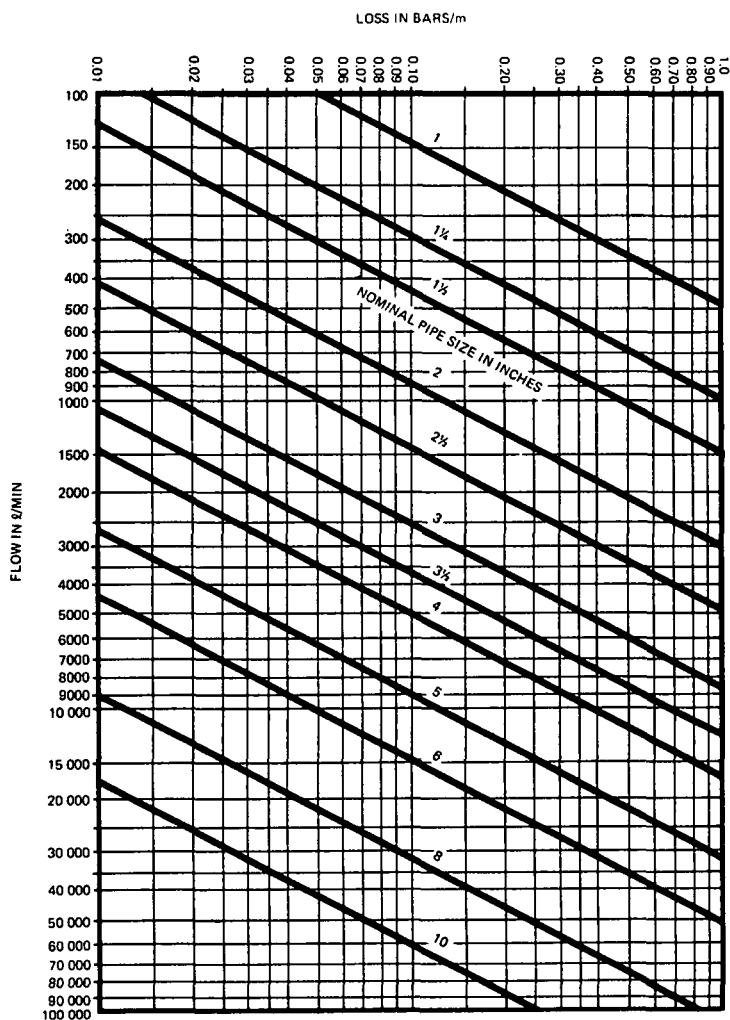
Figure A-7-2(b) Metric. Friction Loss in Schedule 40 Steel Pipe, Hazen &amp; Williams C-120.
