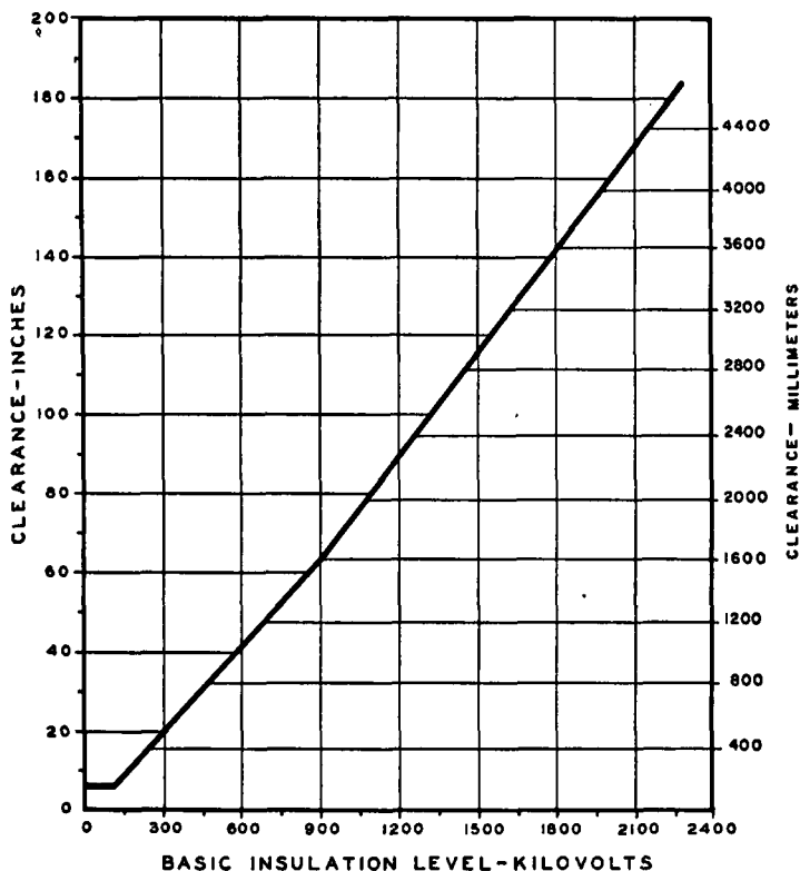
Figure 1-9 Clearance from Water Spray Equipment to Live Uninsulated Electrical Components.
