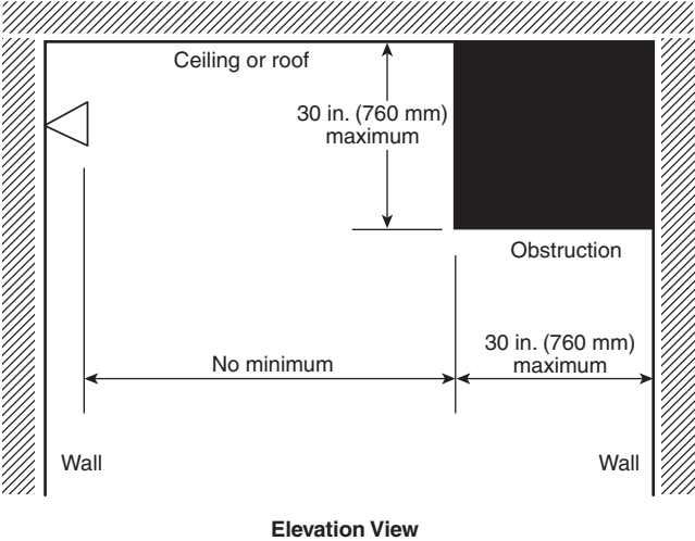
Δ FIGURE 6.4.6.3.7.2(c) Positioning of Sprinkler to Avoid Obstruction Against Wall (Residential Sidewall Sprinklers).
