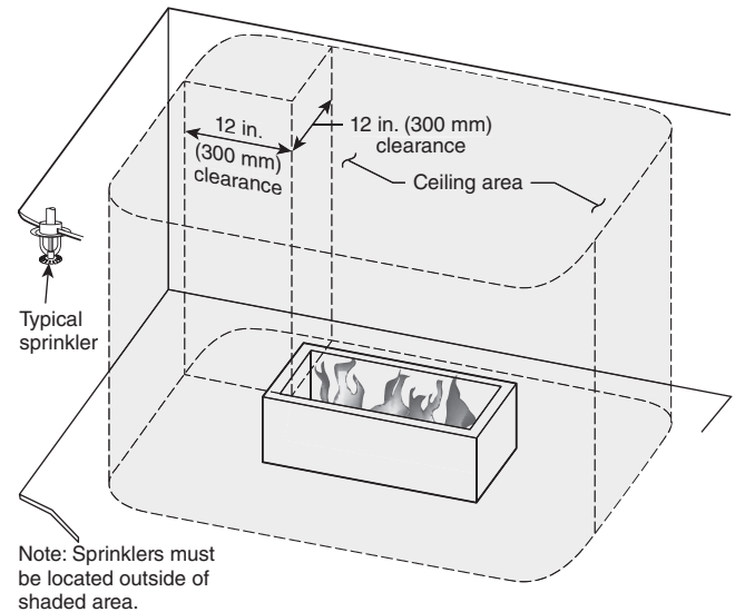
FIGURE A.6.2.3.3(d) Open Fireplace — Intermediate Temperature Sprinkler Location.
