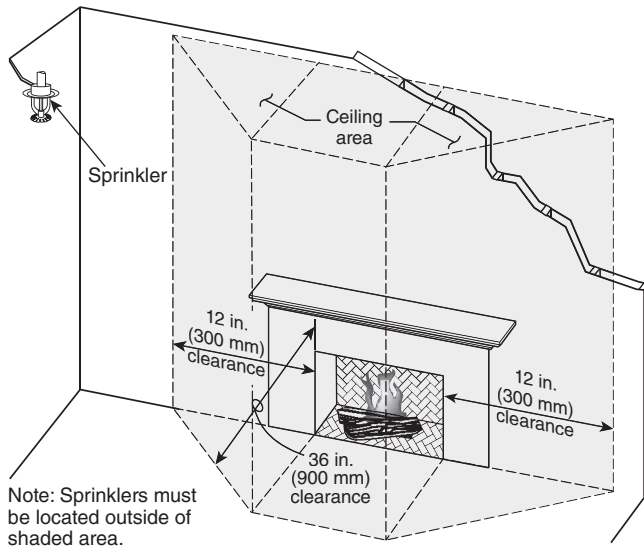
FIGURE A.6.2.3.3(b) Recessed Fireplace — Intermediate Temperature Sprinkler Location.
