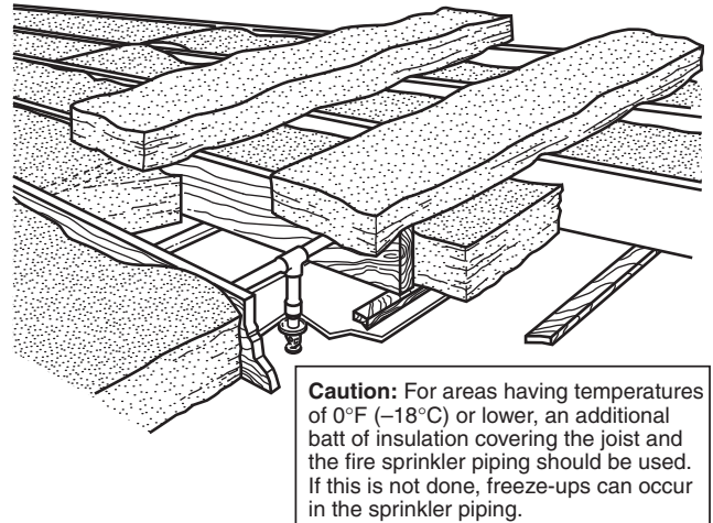
FIGURE A.5.4.2(b) Insulation Recommendations — Arrangement 2.
