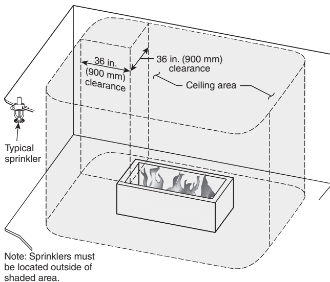
FIGURE A.6.2.3.3(c) Open Fireplace — Ordinary Temperature Sprinkler Location.
