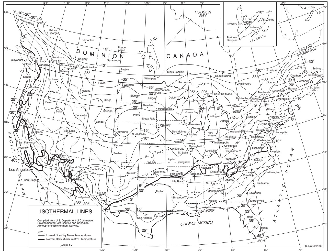
FIGURE A.6.2.4.1(c) Isothermal Lines — Lowest One-Day Mean Temperature (°F). [24:Figure A.10.5.1]
