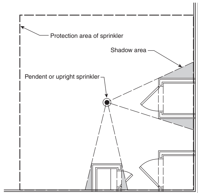
FIGURE A.6.4.6.3.3.1(a) Example of Shadow Areas (SSU/SSP).
