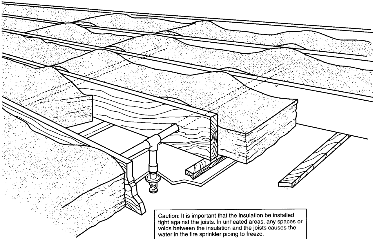
Figure A-4-3.1(a) Insulation recommendations.
