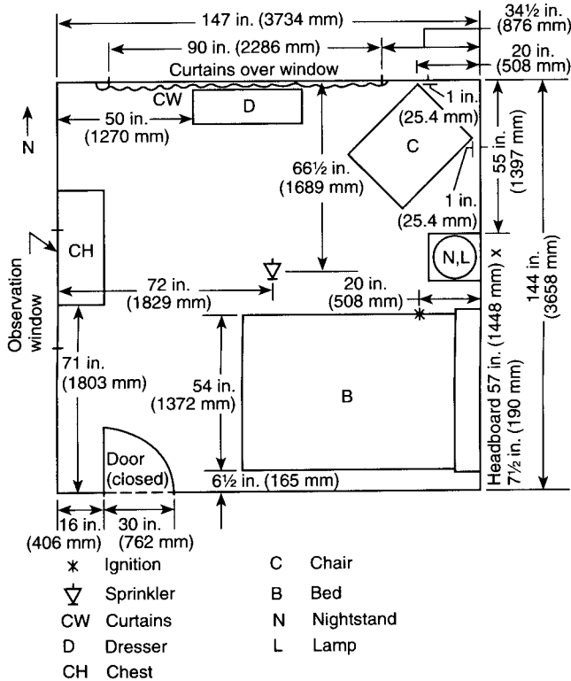
Figure A-1-1(a) Bedroom.
