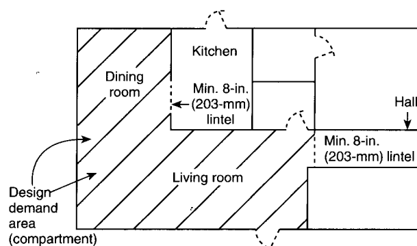
Figure A-4-1.2(a) Sprinkler design areas for typical residential occupancy.
