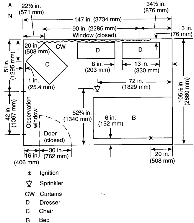
Figure A-1-1(b) Manufactured home bedroom.
