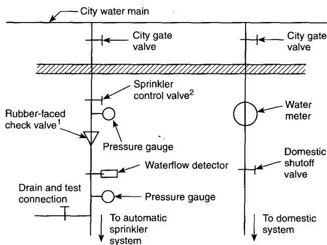
Figure A-2-2(a) Preferable arrangement.
