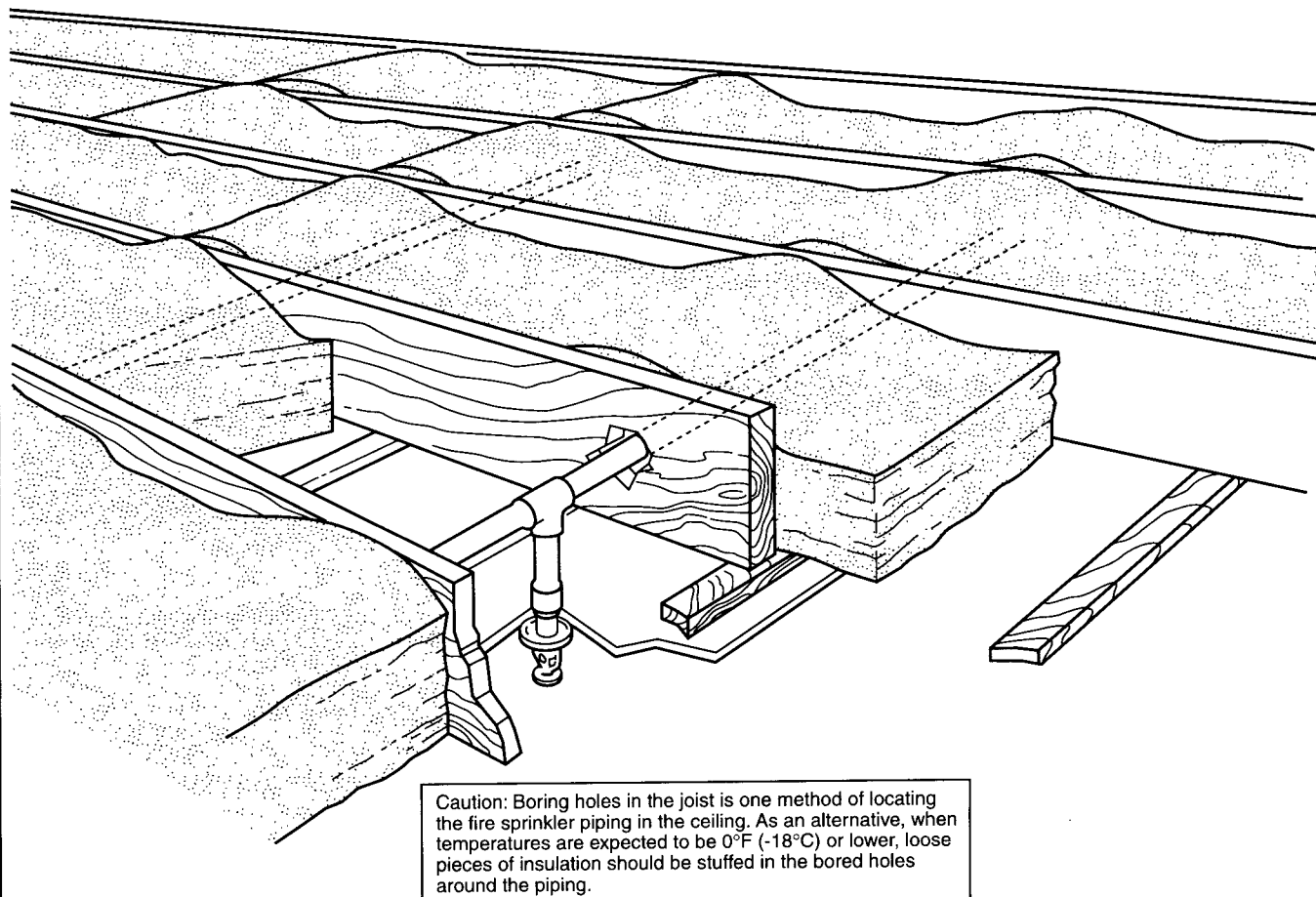
Figure A-4-3.1(c) Insulation recommendations.
