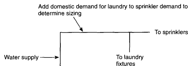
Figure A-2-3(b) Multipurpose pipe system calculation procedure.
