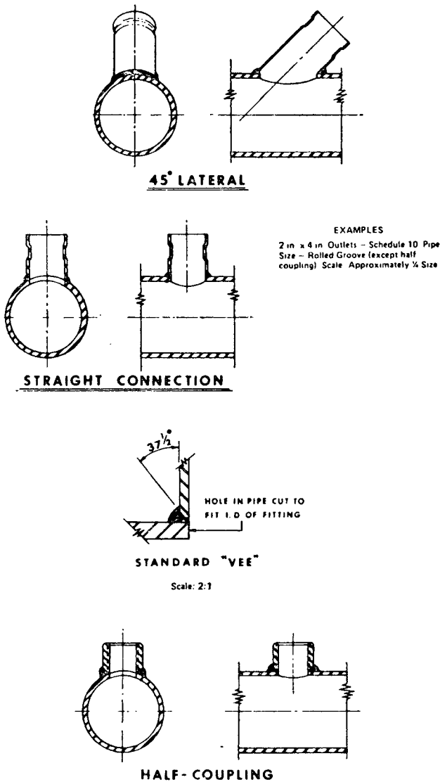
Figure A-3-12.2(b) Welded Branch Connections.
