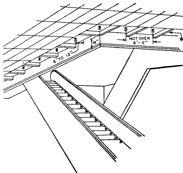
Figure A-4-4.8.2.3 Sprinklers Around Escalators. See 4-4.19.
