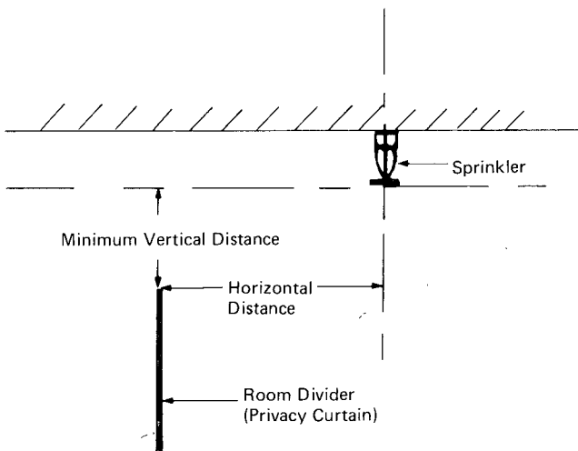
Figure 4-2.5.2 Standard Sprinkler Installed Near Privacy Curtain.
