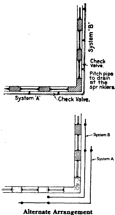
Figure 6-2.1.4 Arrangement of Check Valves.
