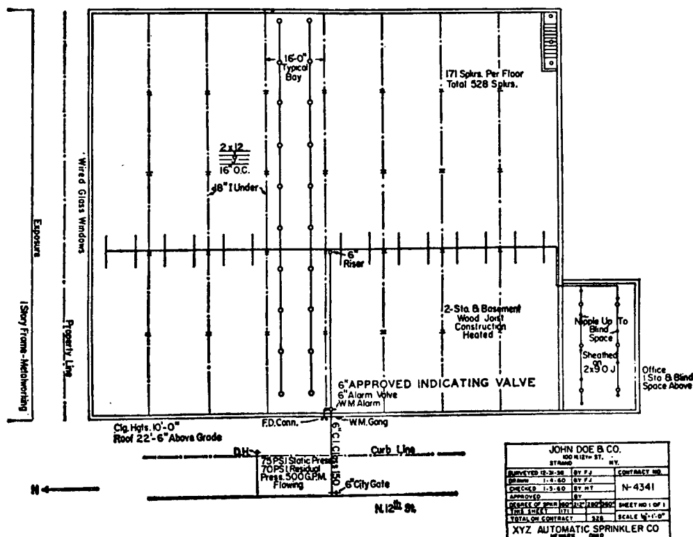
Figure A-1-9 Typical Preliminary Plan.
