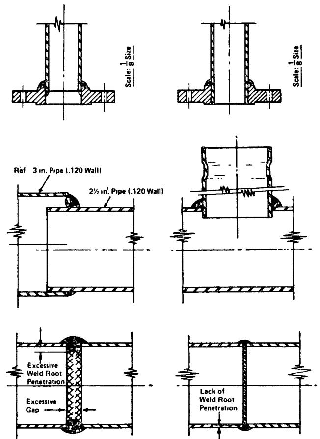
Figure A-3-12.2(c) Unacceptable Weld Joints.
