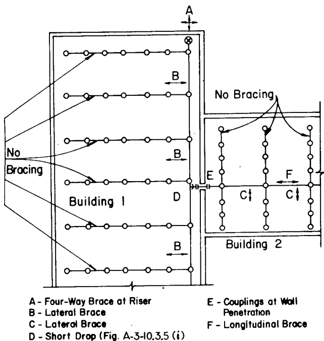
Figure A-3-10.3.5(a) Earthquake Protection for Sprinkler Piping.
