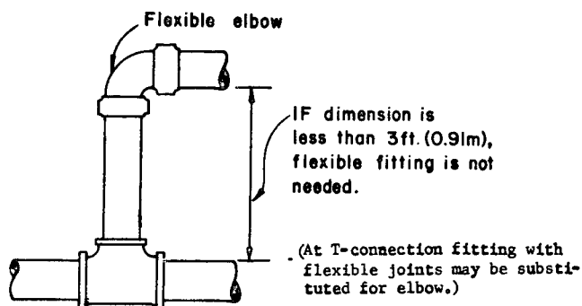
Figure A-3-10.3.2(b) Detail at Short Riser.
