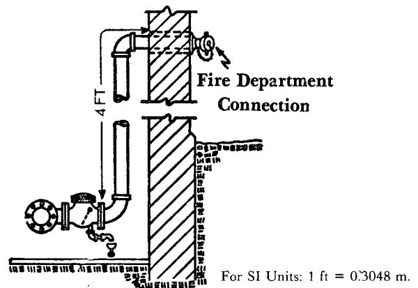
Figure A-3-10.1.2 Minimum Clearance to Avoid Freezing
