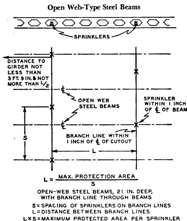
Figure 4-2.4.4 Location of Branch Lines and Sprinklers.
