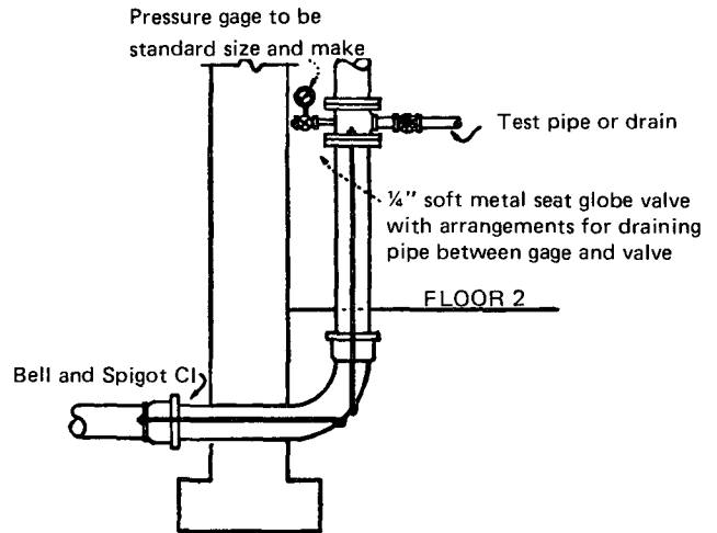
Figure A-2-9.1 Test Pipe on Water Supply with Outside Control. Also applicable to an interior riser.
