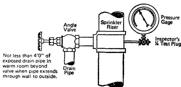
Figure 3-11.2 Drain Connection for Sprinkler Riser.
