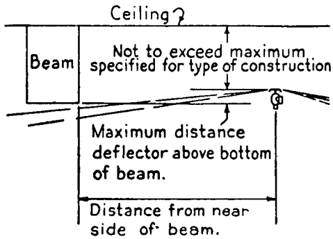
Figure 4-2.4.6 Position of Deflector, Upright, or Pendant, When Located Above Bottom of Beam.
