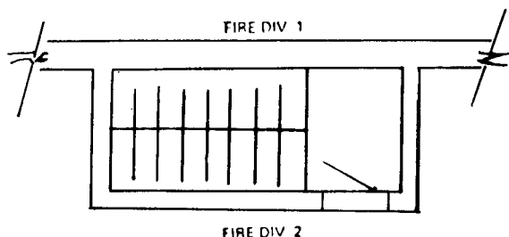
Figure A-4-4.8.2.4(b) Noncombustible Stair Shaft Serving One Fire Section.
