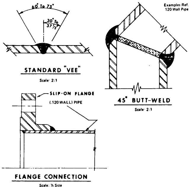
Figure A-3-12.2(a) Butt-Weld Joints and Flange Connection.
