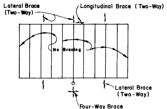
Figure A-3-10.3.5(c) Typical Location of Bracing on a Gridded System.
