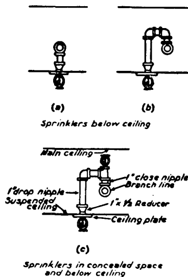
Figure 3-8.4 Pendent Sprinklers at Suspended Ceiling.
