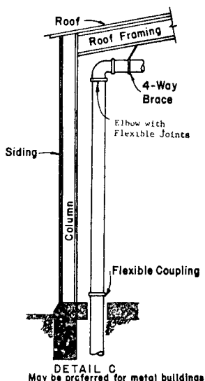
Figure A-3-10.3.2(a) Riser Details.
