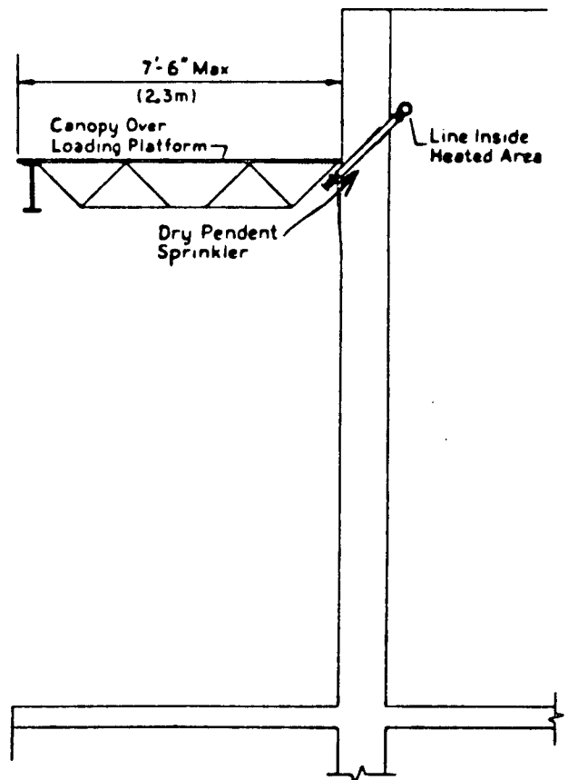
Figure 5-5.6 Dry Pendent Sprinklers for Protection of Covered Platforms, Shipping Docks, and Similar Areas.
