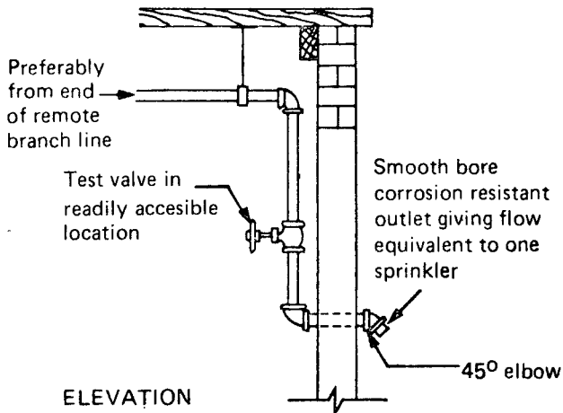
Figure A-3-9.1.1 System Test Pipe on Wet-Pipe System.
