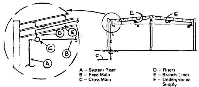
Figure A-3-2 Building Elevation Showing Parts of Sprinkler Piping System.
