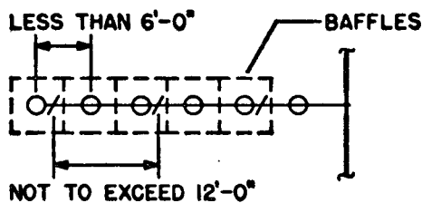
Figure A-3-15.5.3 Distance Sprinkler to Hanger.
