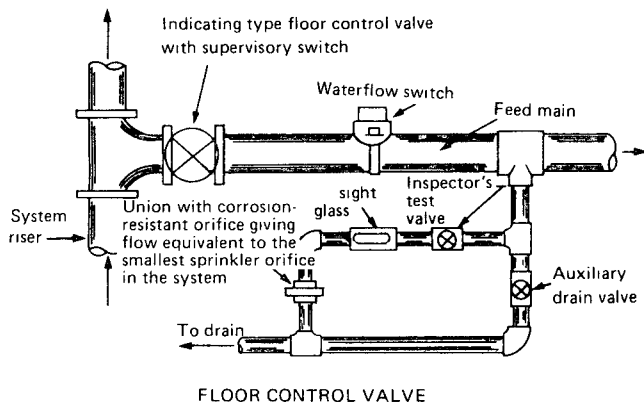
Figure A-3-9.1.2 Floor Control Valve.
