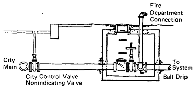
Figure A-3-14.2.5 Pit for Gate Valve, Check Valve and Fire Department Connection.
