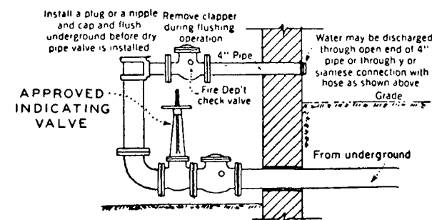
Figure A-1-11.1 Methods of Flushing Water Supply Connections.
