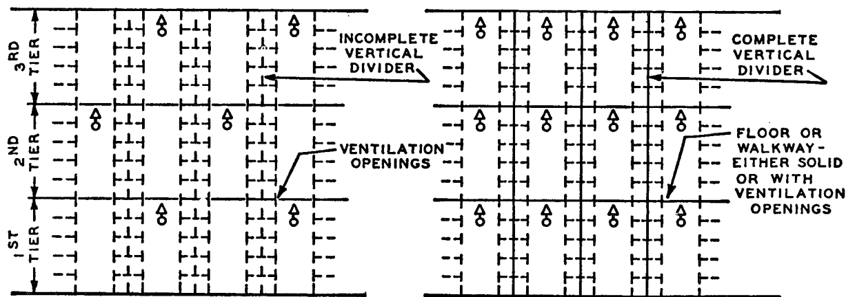
Figure 4-4.12 Sprinklers In Multitier Library Bookstacks.
