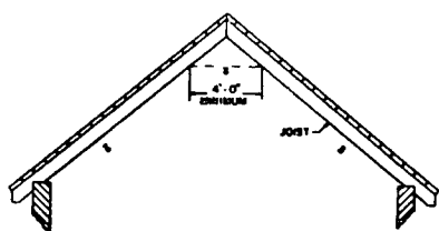
Figure 4-4.5.4 Desirable Horizontal Clearance for Sprinklers at Peak of Pitched Roof.
