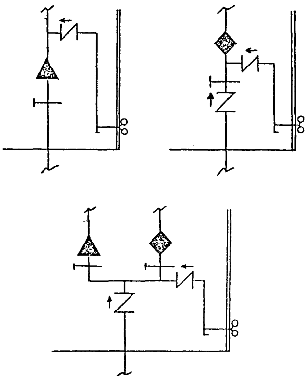
Figure A-3-14.2 Examples of Acceptable Valve Arrangements.
