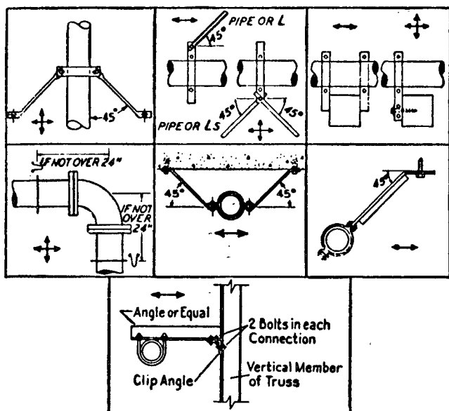
Figure A-3-10.3.5.1(a) Acceptable Types of Sway Bracing.
