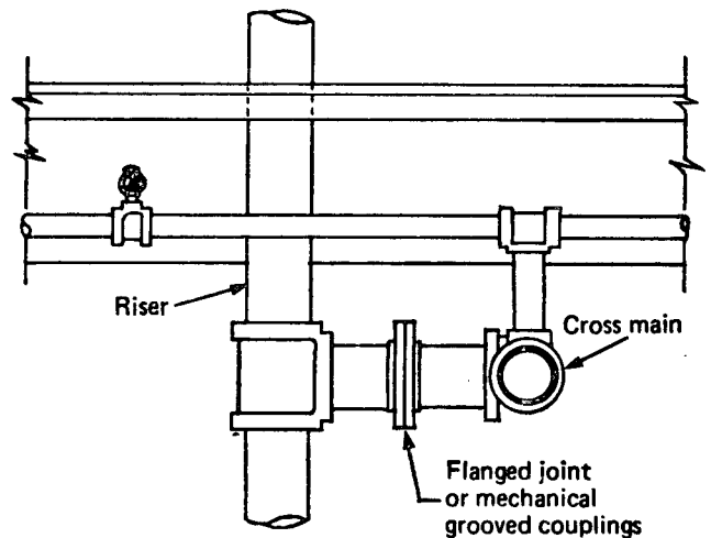
Figure A-3-13.1.5 One Arrangement of Flanged Joint at Sprinkler Riser.
