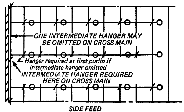
Figure A-3-15.6.1(B) Hanger Omission on Side Feed System.
