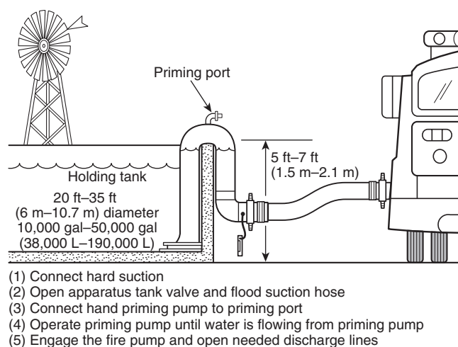
FIGURE B.7 Drafting Procedure for Farm Holding Tanks.
