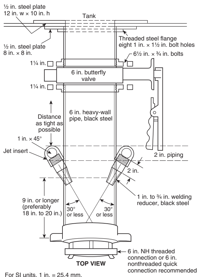
FIGURE C.12.2.2(a) Peripheral Jet-Assist Installation (Top View).
