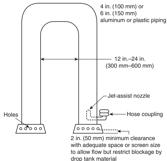
FIGURE C.12.2.3(a) Jet-Assist Transfer Siphon.
