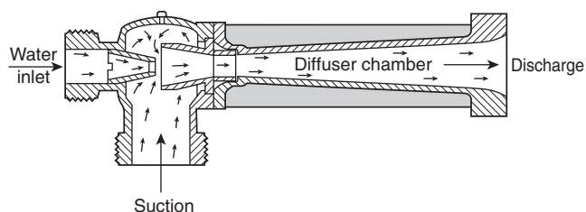
FIGURE C.12.2.4(c) Cross-Section of Water Ejector Showing Motive Line Water Inlet, Suction Inlet, and Supply Line Discharge.
