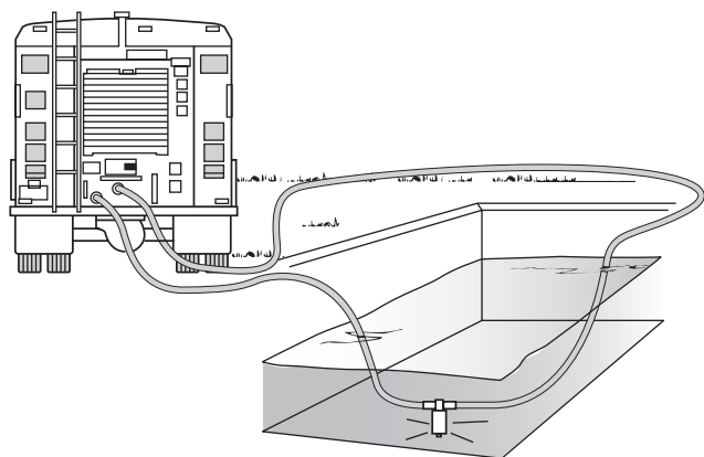
FIGURE C.12.2.4(b) Ejector Use from the Street to a Back Yard Swimming Pool.
