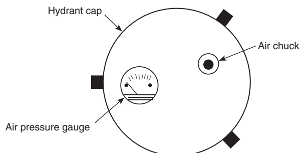
FIGURE A.8.4.6(b) Cap Design for Air Injection System.
