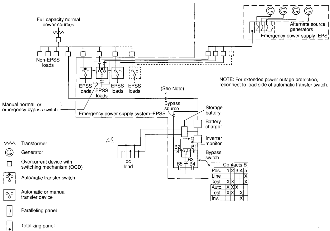
Figure B-4 Typical composite emergency power supply system.
