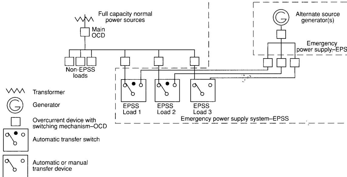
Figure B-1 Typical rotating emergency power supply system.
