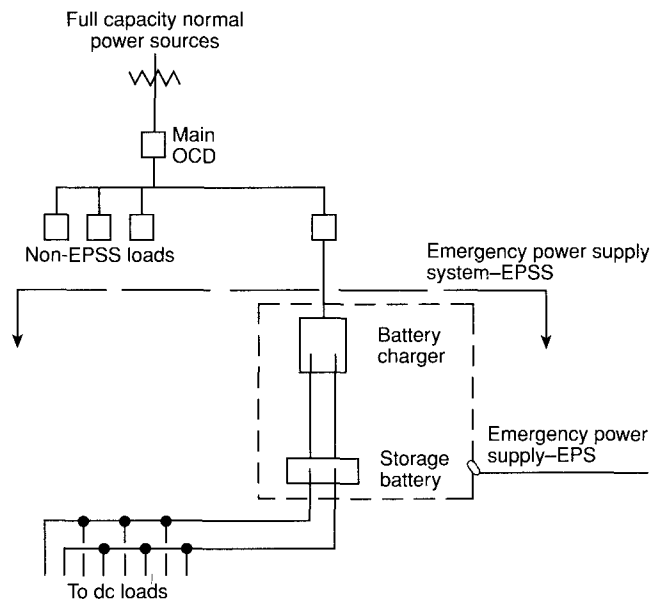
Figure B-3 Typical uninterruptible power supply system (UPS).
