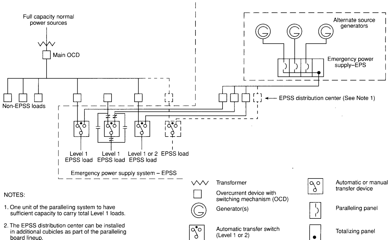
Figure B-2 Typical multiple unit emergency power supply system.
