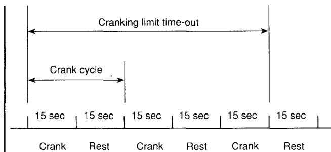
Figure A-3-5.4 Diagram of cranking cycles.
