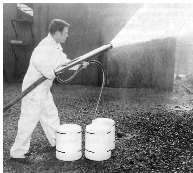
FIGURE A.3.3.6.1 Air Foam Hose Nozzle with Built-in Eductor.
