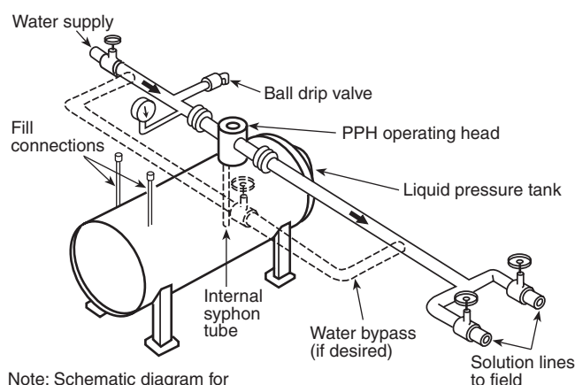
FIGURE A.3.3.23(a) Typical Arrangement of Pressure Proportioning Tank.
