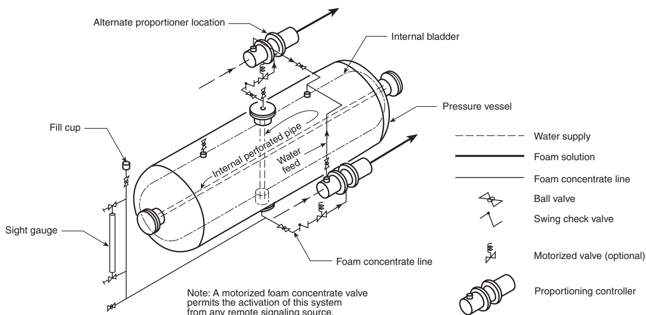
FIGURE A.3.3.23(b) Diaphragm (Bladder) Proportioning Tank.
