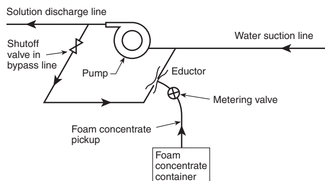
FIGURE A.3.3.27(a) Around-the-Pump Proportioner.
