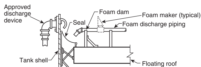
DETAIL A — Top-of-seal application Foam discharge above mechanical shoe seal
