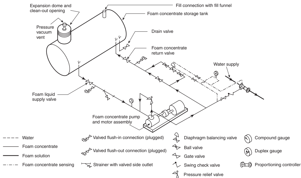
FIGURE A.3.3.25.1 Balanced Pressure Proportioning (Pump-Type) with Single Injection Point.
