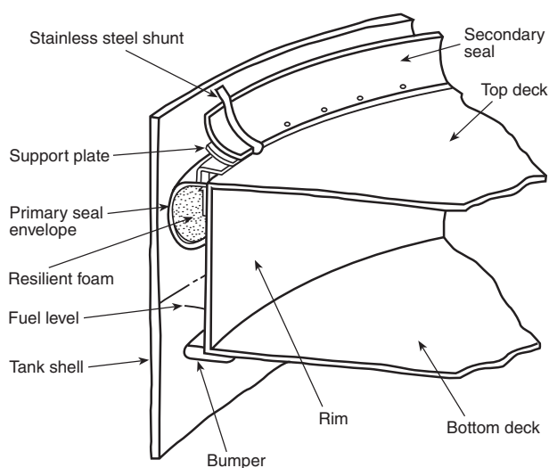
FIGURE 5.3(c) Double Seal System for Floating Roofs.
