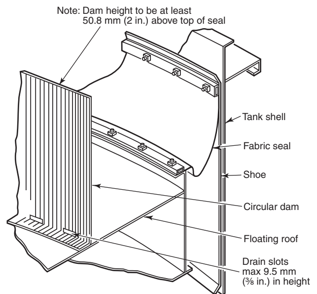
FIGURE 5.3.5.4.5 Typical Foam Dam for Floating Roof Tank Protection.
