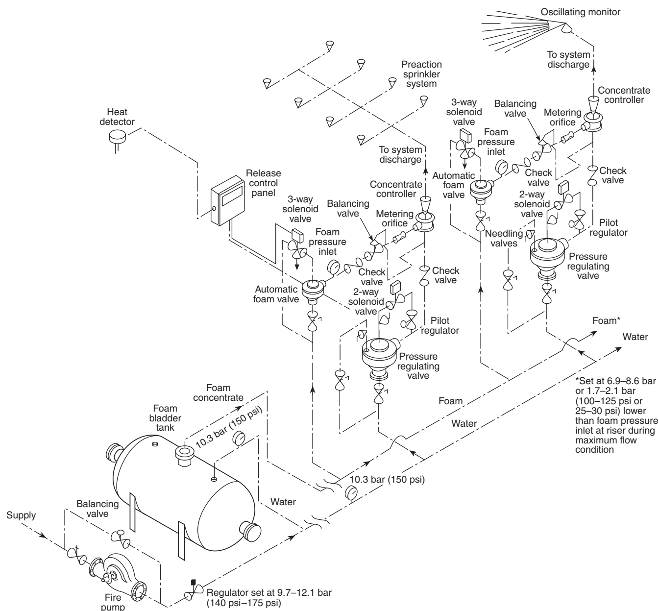
FIGURE A.3.3.25.1.1(b) In-Line Balanced Pressure (Bladder Tank Type) Proportioning with Multiple Injection Points.
