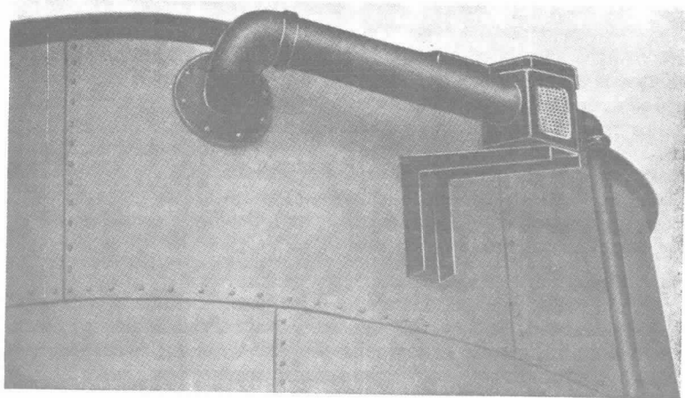
Figure A-3-2.5.2(a) Air Foam Maker in Horizontal Position at Top of Storage Tank.
