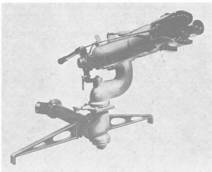
Figure A-3-1.2(e) Portable Foam-Water Monitor.
