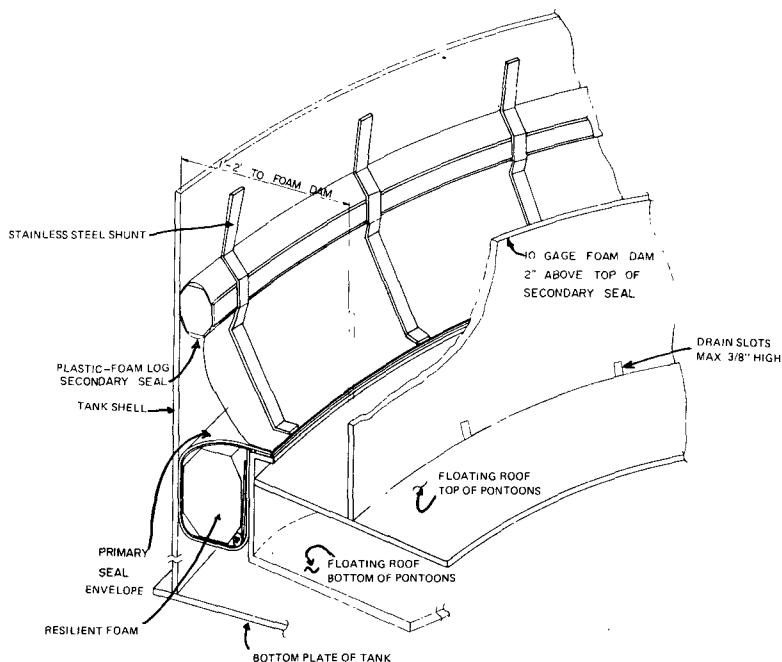
Figure A-3-2.11.1(d) Double Seal System for Floating Roofs Using a Plastic-Foam Log (Secondary Seal).
