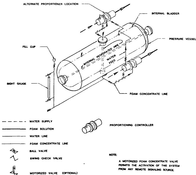
Figure A-1-4(i) Diaphragm (Bladder) Proportioning Tank.
