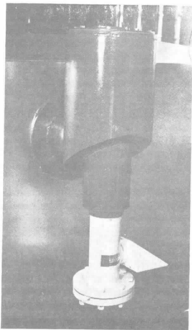
Figure A-3-2.5.2(b) Foam Chamber and Foam Maker.
