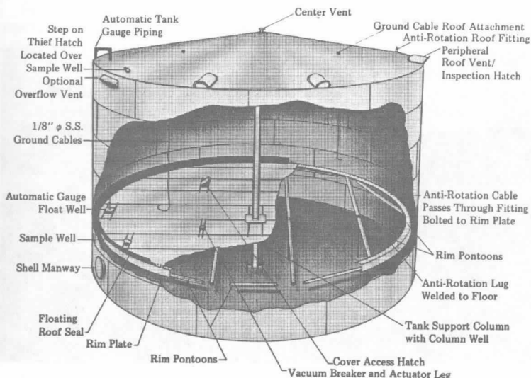
Figure A-3-2.11.2 Typical Covered Floating Roof Tank.
