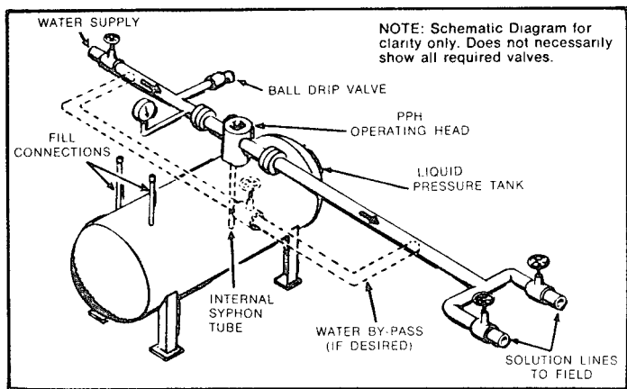
Figure A-1-4(h) Typical Arrangement of Pressure Proportioning Tank.
