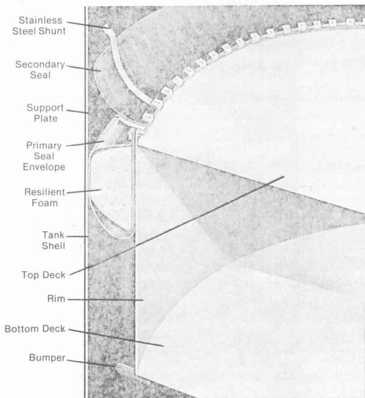
Figure A-3-2.11.1(c) Double Seal System for Floating Roofs.
