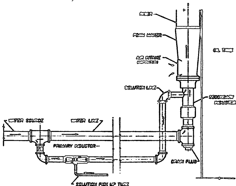
Figure A-1-4(d) Air Foam Auto-Eduction System. Solution Pick-up Tube Picks up Concentrate from its Container.
