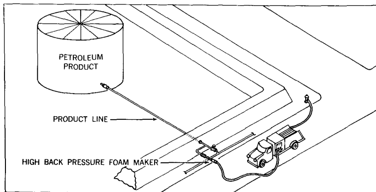
Figure A-3-2.2(d) Semifixed Subsurface Foam Installation.
