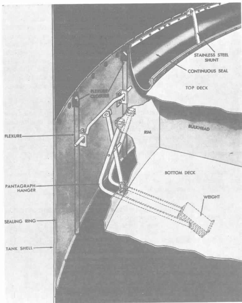
Figure A-3-2.11.1(a) Pantograph-type Seal Open Top Floating Roof Tank.
