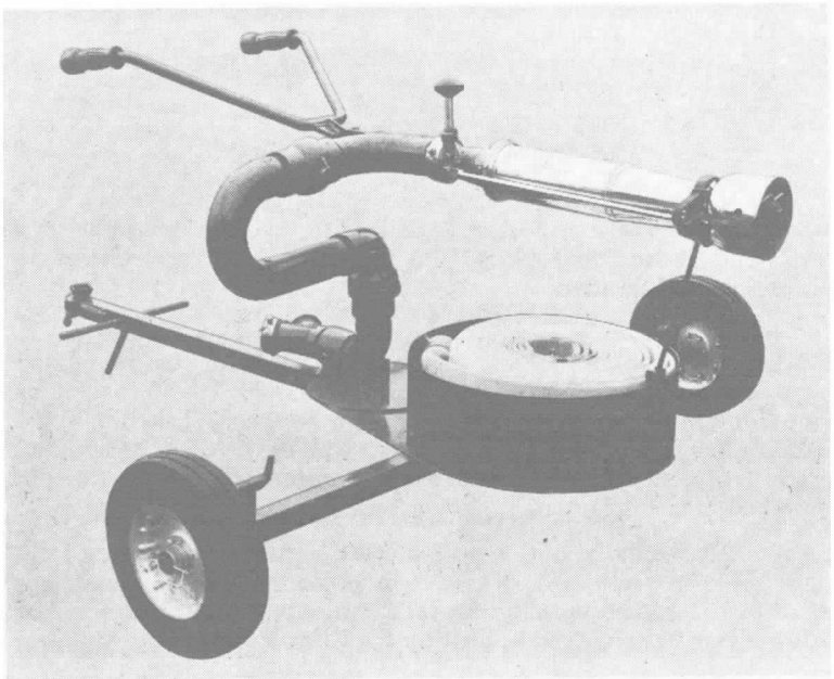
Figure A-3-1.2(d) Wheeled Portable Foam-Water Monitor.
