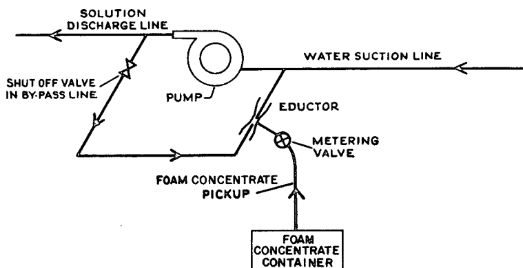
Figure A-1-4(e) Around-the-Pump Proportioner.
