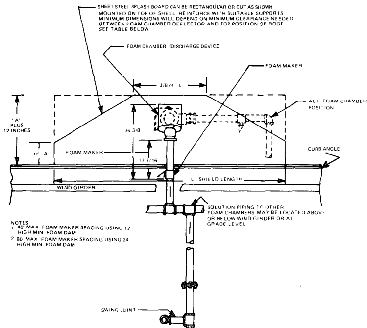
Figure A-3-2.11.1(e) Typical Foam Splash Board for Discharge Devices Mounted Above the Top of the Shell. (Continued)
