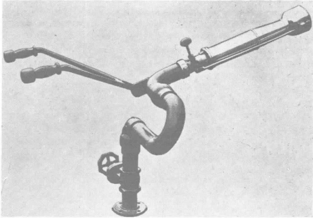
Figure A-3-1.2(c) Adjustable Straight Stream-to-Spray Foam-Water Monitor.
