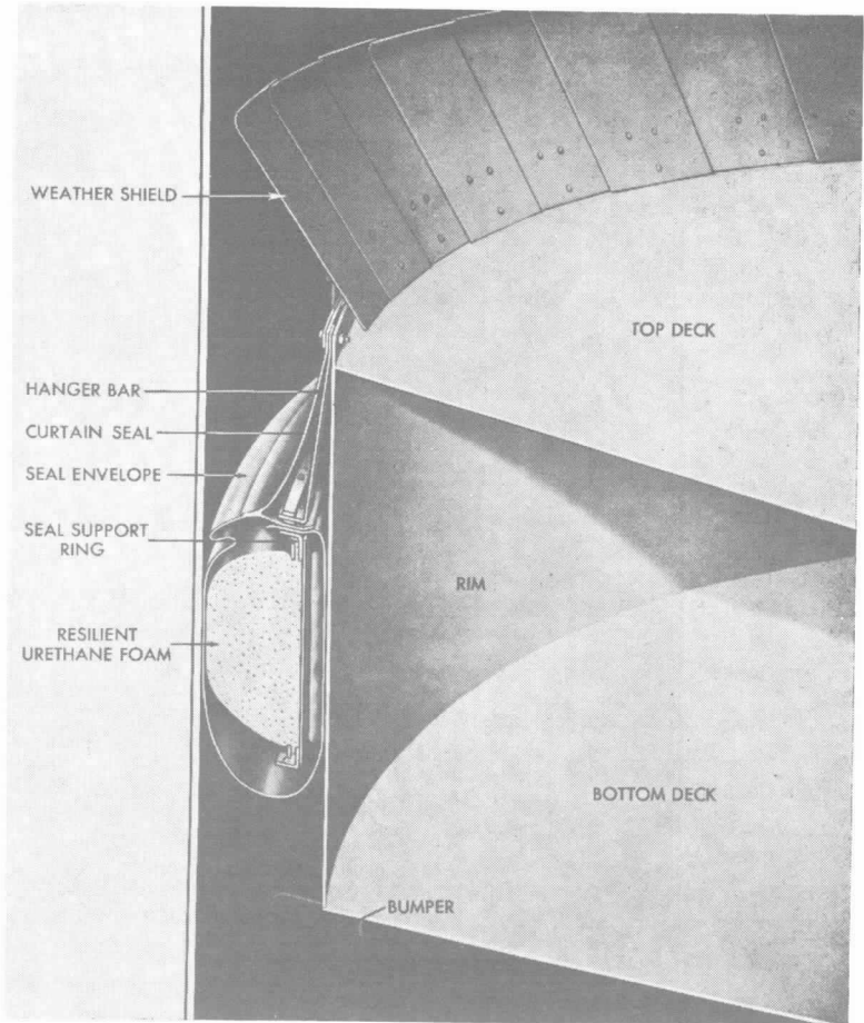
Figure A-3-2.11.1(b) Tube Seal Open Floating Roof Tank.
