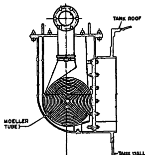
Figure A-3-2.2(a) Cross-section of a Moeller Tube Chamber. Tube is designed to unroll and fall to oil level. Foam flows through interstices in tube.
