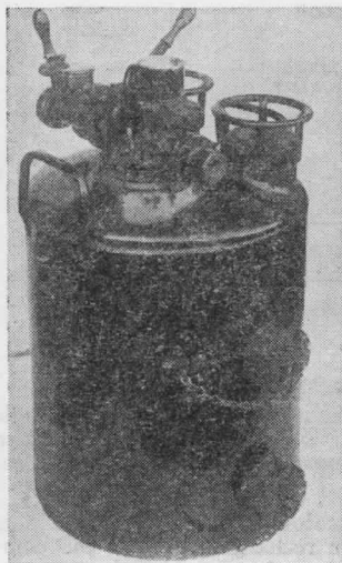
Fig. A-11-55.31A. Pressure Proportioner, Compartmented Single Tank.
