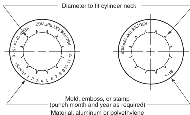
FIGURE A.7.13 Design of a Verification-of-Service Collar.
