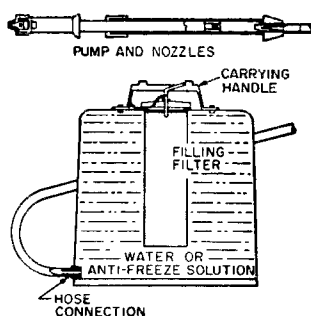
Figure D-4-1.4 Pump Tank Back Pack Fire Extinguisher.
