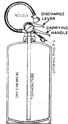
Figure D-4-5(a) Stored Pressure Dry Chemical Extinguisher.
