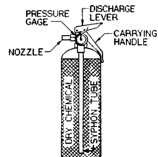
Figure D-4-5(c) Stored Pressure Dry Chemical with Fixed Nozzle.
