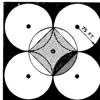
Figure E-3-3 The Dotted Squares Show the Maximum Area (11,250 sq ft) (1,045 m 2 ) that an Extinguisher Can Protect within the Limits of the 75-ft (22.7-m) Radius.
