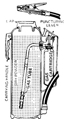
Figure D-4-6.1 Dry Powder Extinguisher.
