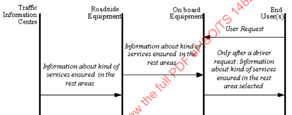
Figure 23 — Rest area information: data flow
