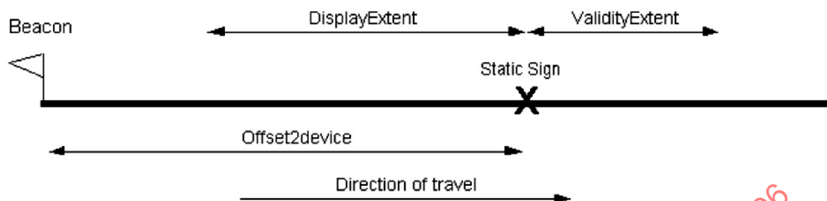
Figure 10 — Static road signs information: structure
