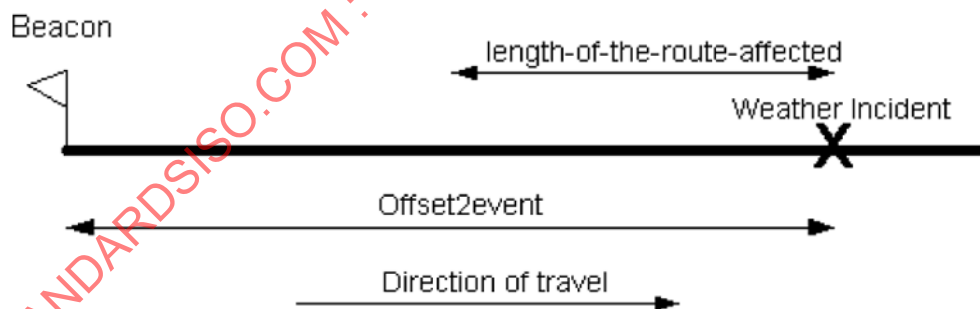
Figure 20 — Weather information: structure
