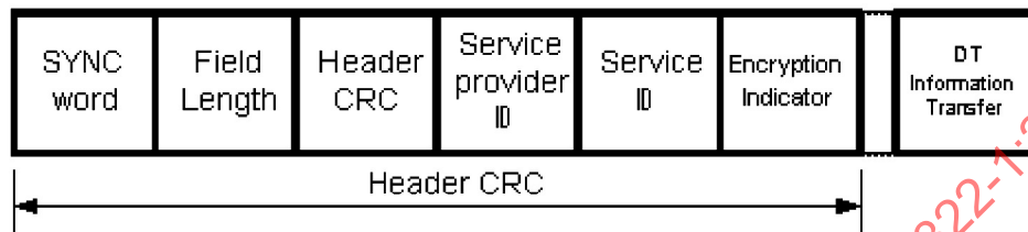
Figure 2 — Header CRC
