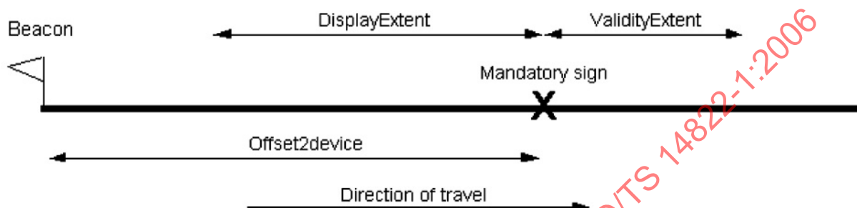
Figure 8 — Static road signs mandatory: structure
