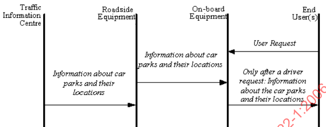
Figure 27 — Parking information: data flow
