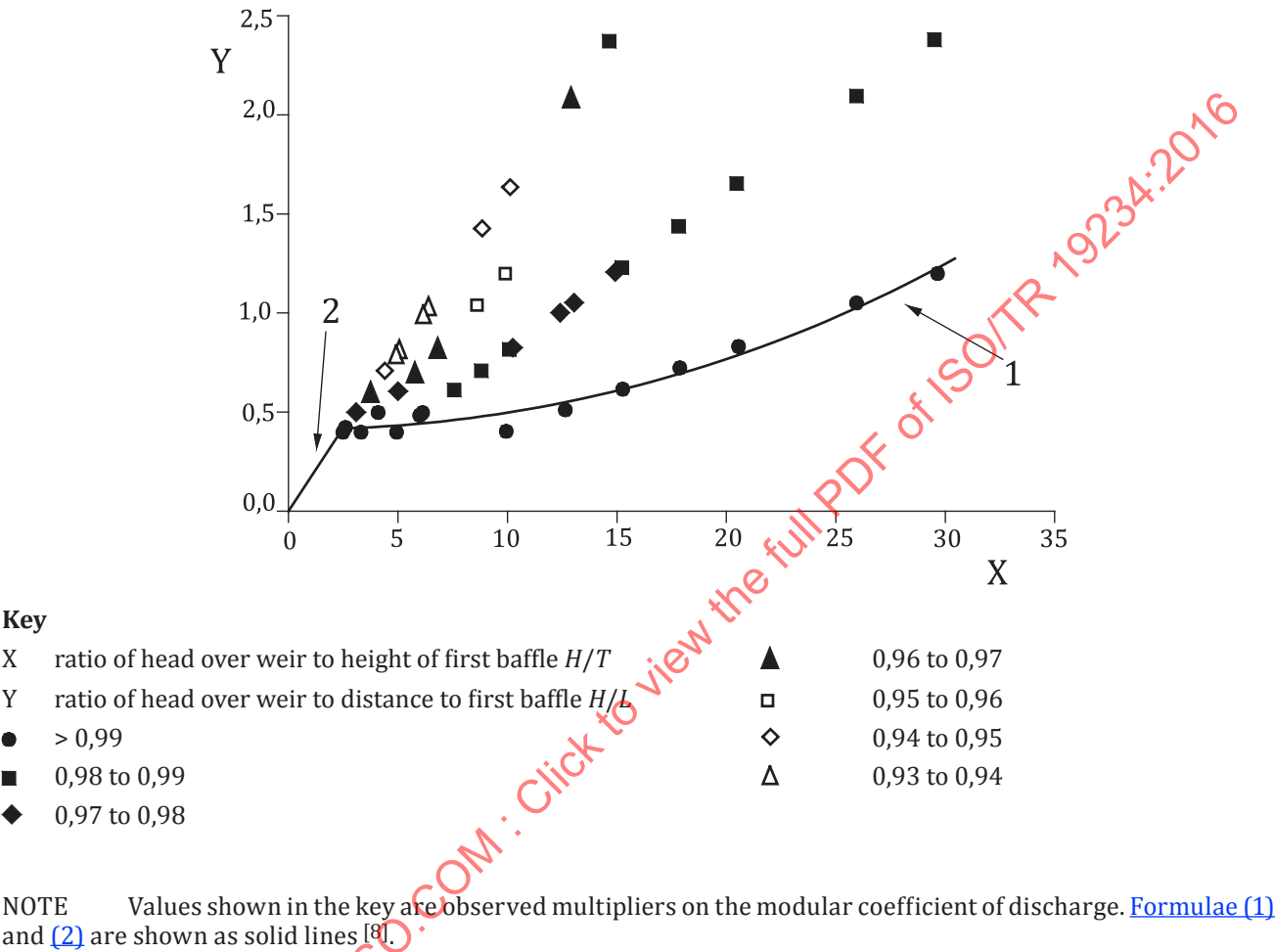
Figure 4 — Hydrometric effects of near-crest baffles
