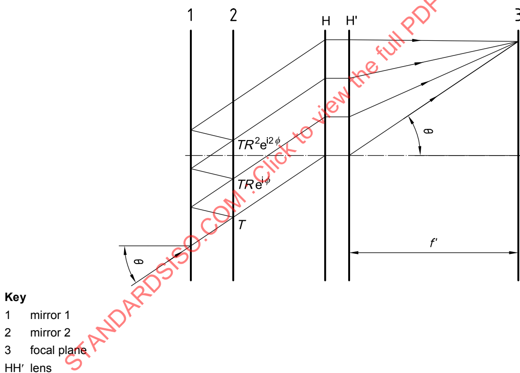
Figure 20 — Fringe formation by a multiple-beam Fabry-Perot interferometer
