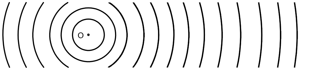
Figure 3 — Spherical waves
