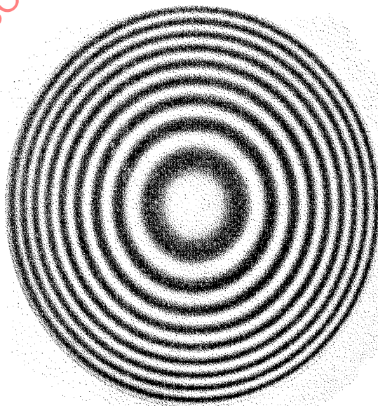
Figure 13 — Newton's rings
