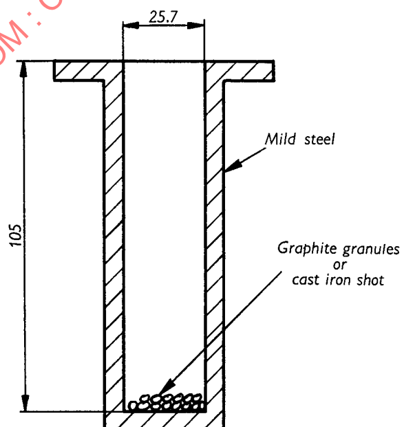
FIG. 2. — Mild steel vessel for heating the test piece
