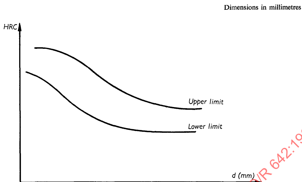
FIG. 6 (a) — Specification by two limiting curves
