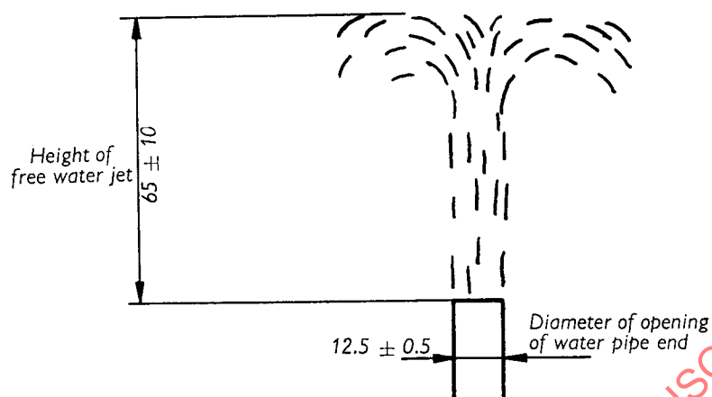
FIG. 4. — Water pipe end
