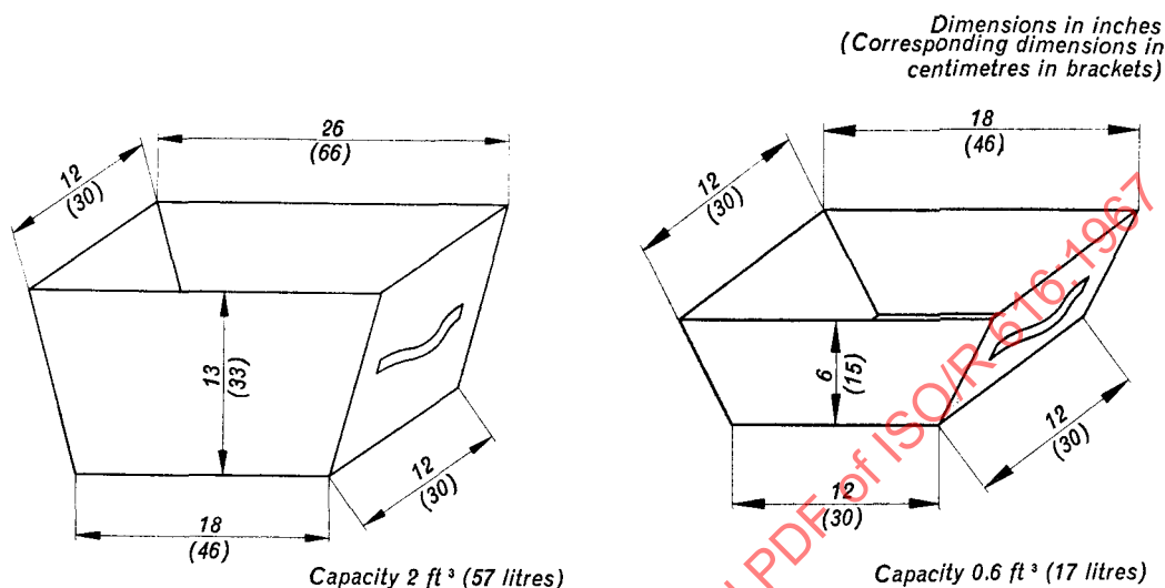
FIG. 3. — Containers for use in determination of shatter indices.
