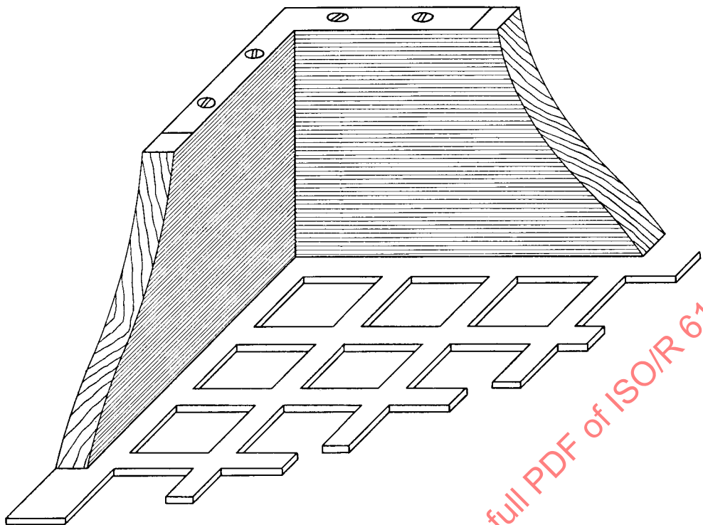
FIG. 2. — Detail of sieve for determination of shatter indices.
