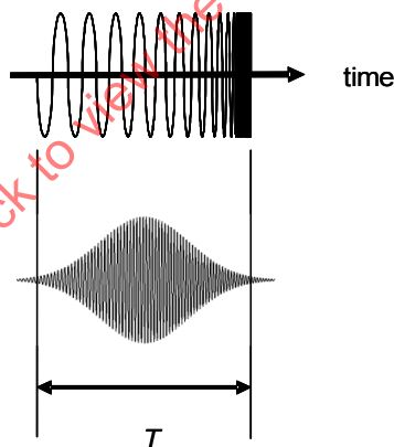
Figure 16-15—Graphical view of a CoU pulse
