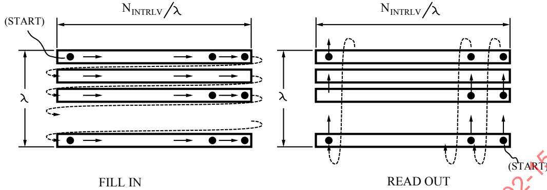
Figure 22-12—Interleaver
