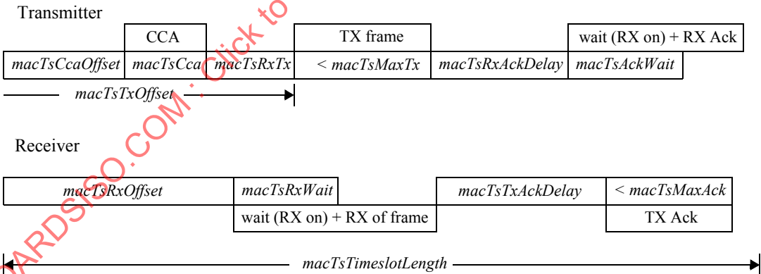
Figure 6-30—Timeslot diagram of acknowledged transmission
