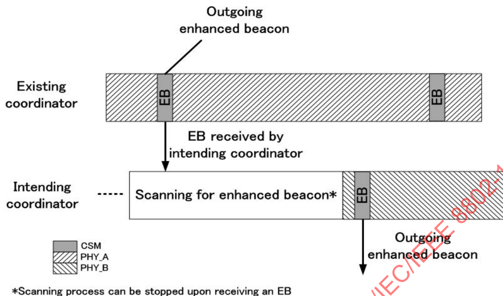
Figure 6-76—Inter-PHY mode coexistence in a nonbeacon-enabled PAN
