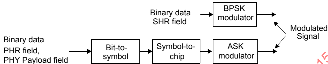
Figure 14-1—ASK reference modulator block diagram
