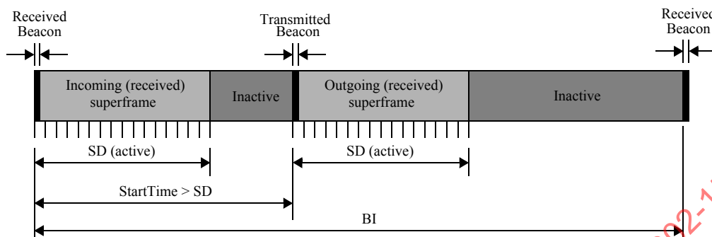
Figure 6-2—The relationship between incoming and outgoing beacons
