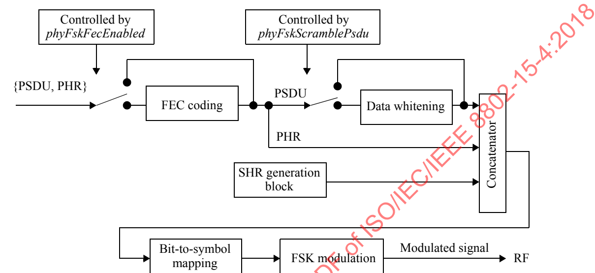
Figure 20-7—SUN FSK reference modulator
