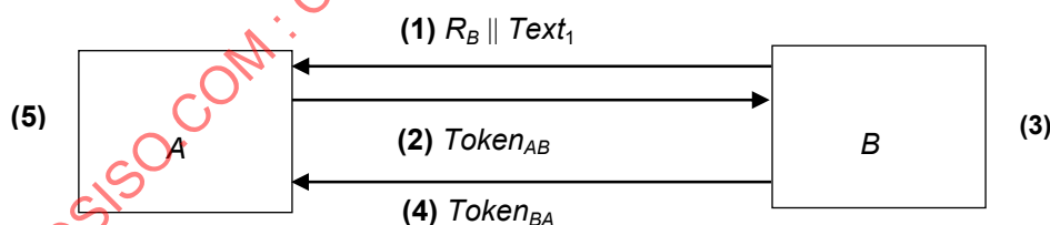
Figure 4 — Mechanism 4 — Three-pass authentication
