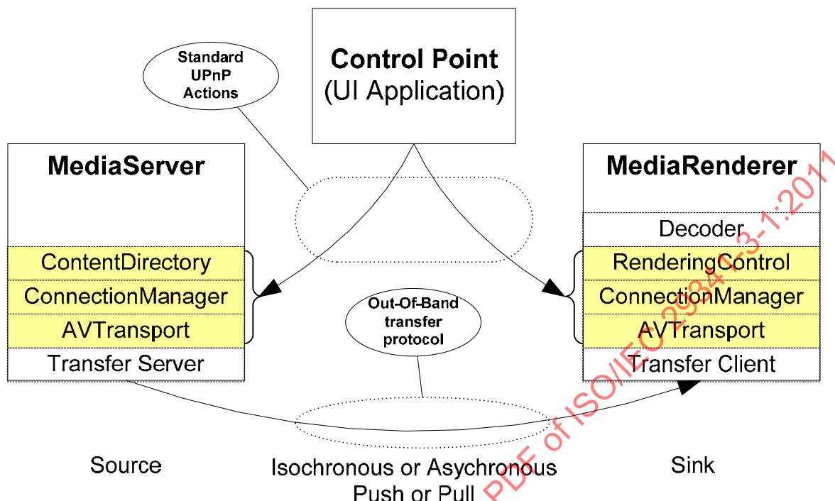
Figure 3 — General Device Architecture aka the 3-Box model
