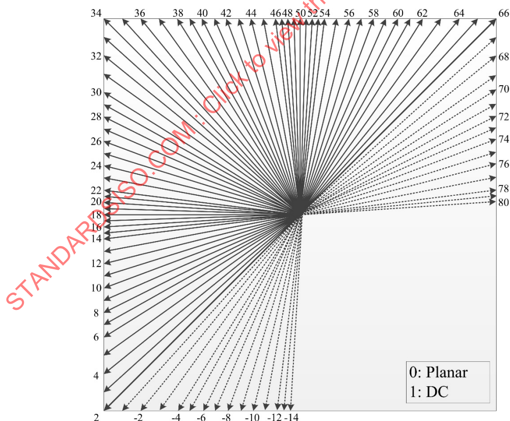
Figure 9 – Intra prediction directions
