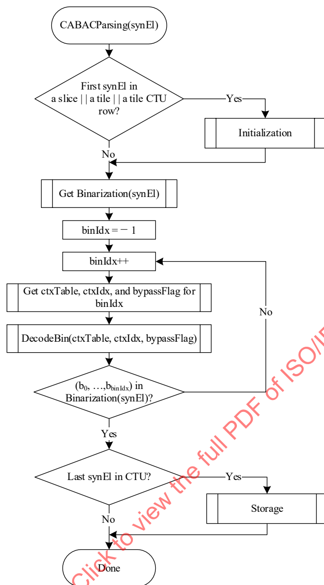
Figure 11 – Flowchart of CABAC parsing process for a syntax element synEl
