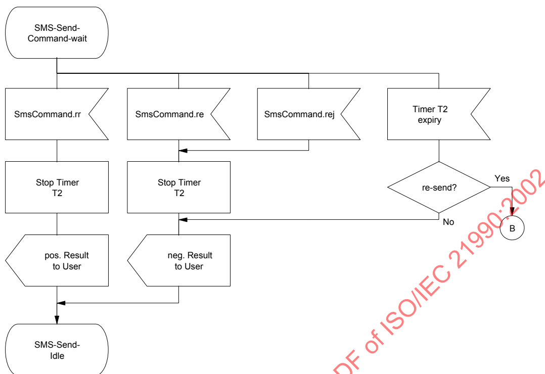
Figure C.1 - Sending User PINX SDL (sheet 2 of 3)
