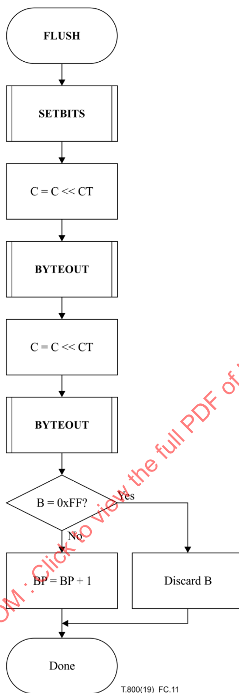
Figure C.11 – FLUSH procedure
