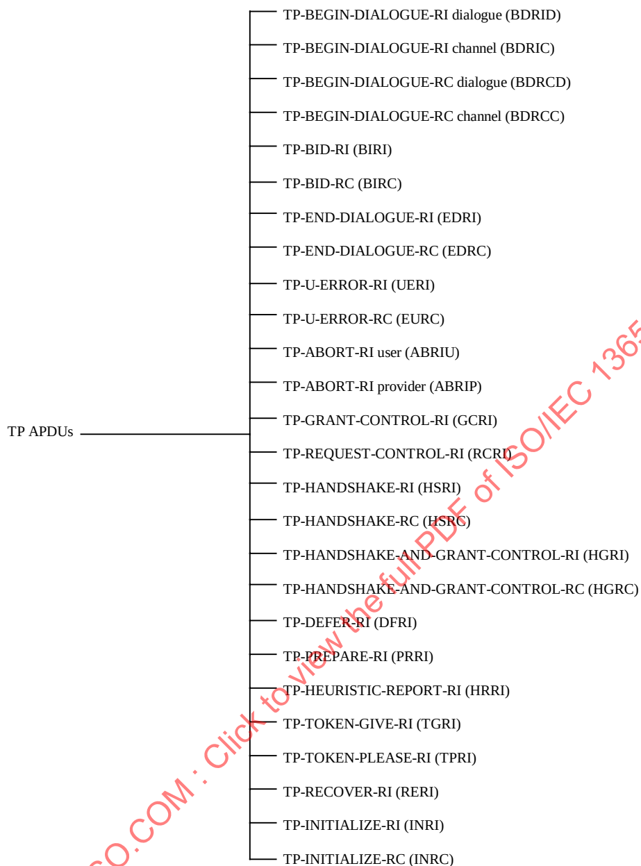
Figure 11 TP APDUs
