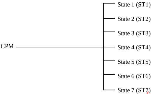
Figure 16 CPM
