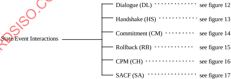
Figure 9 State/Event Interactions
