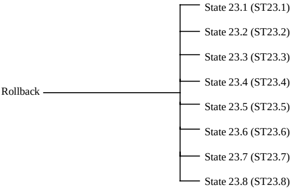
Figure 15 Rollback
