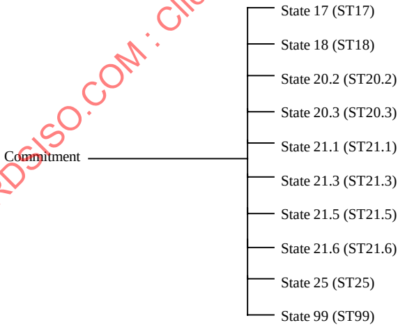
Figure 14 Commitment
