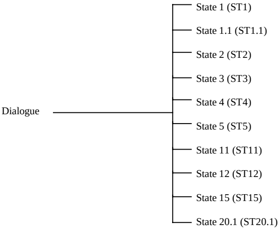
Figure 12 Dialogue
