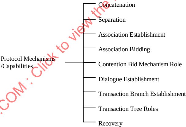
Figure 4 Protocol Mechanisms / Capabilities
