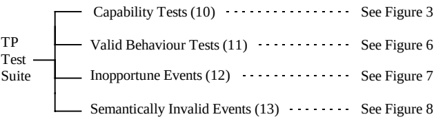
Figure 2 Top-level structure of TP Test Suite
