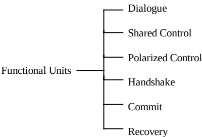
Figure 5 Functional Units
