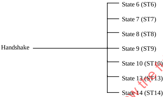
Figure 13 Handshake
