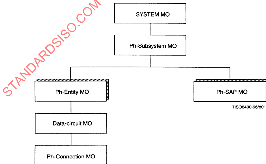
Figure 1 – Physical Layer Containment Hierarchy
