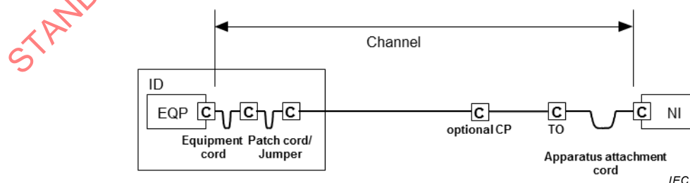
Figure 10 – Transmission performance of a channel
