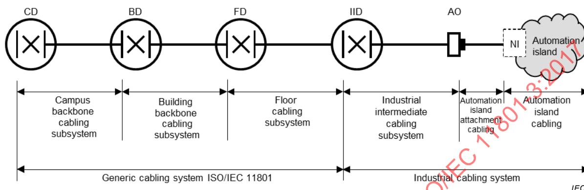
Figure A.2 – Combined structure of generic and industrial cabling system using an IID
