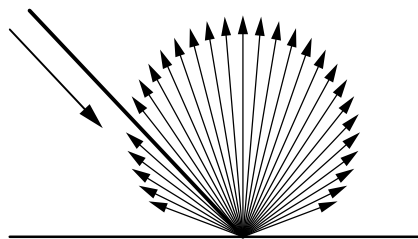
Figure 25 — Diffuse reflection
