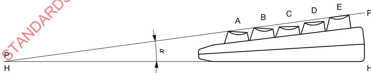
Figure 6 — Keyboard slope
