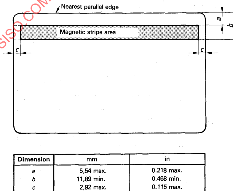
Figure 1 — Location of magnetic stripe area for tracks 1 and 2
