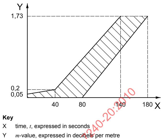
Figure F.2 — Limits for m against time, t , fire TF4
