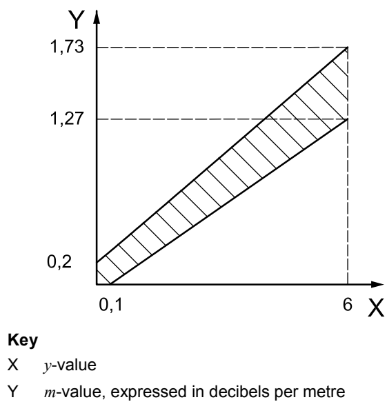
Figure F.1 — Limits for m against y , fire TF4
