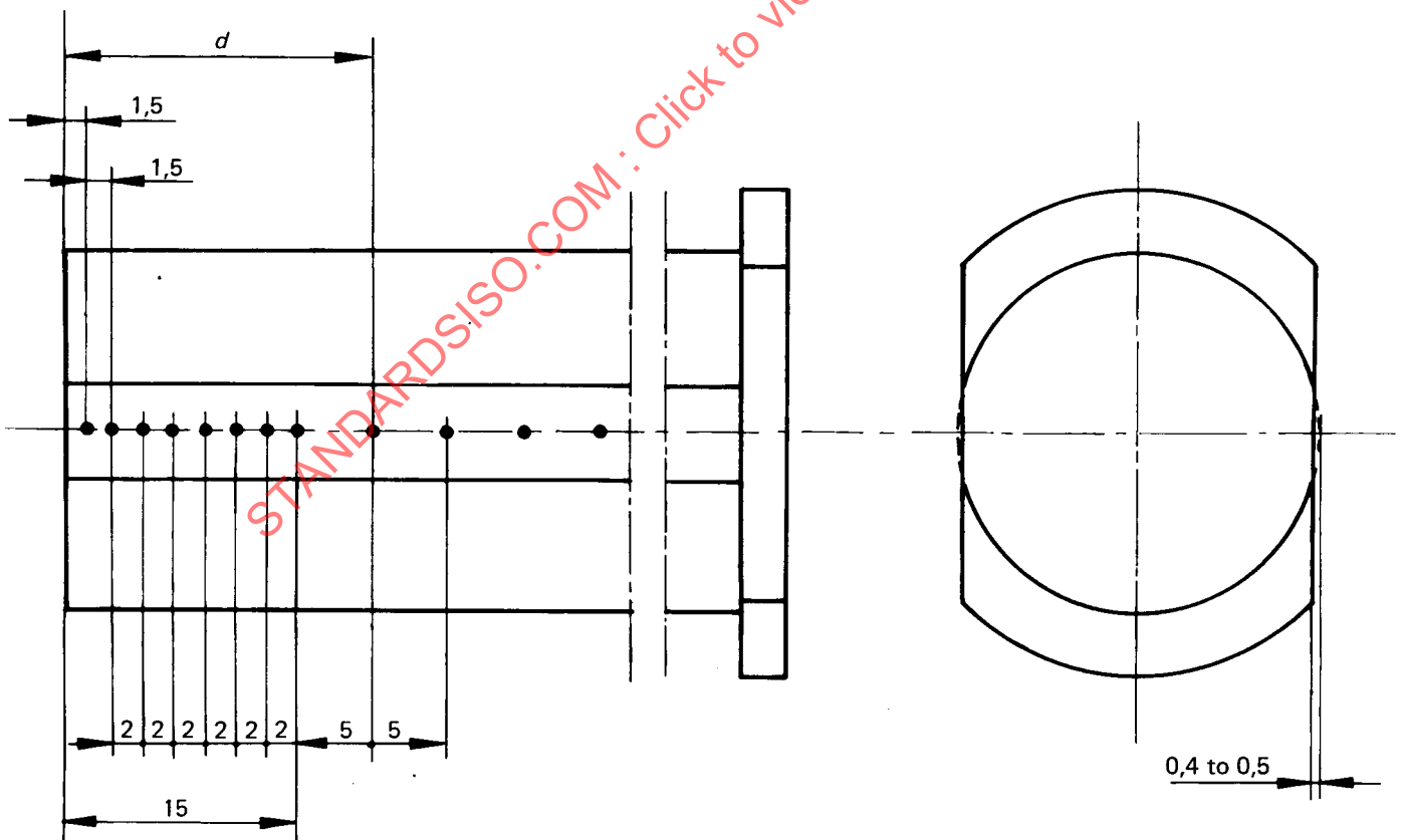
FIGURE 6 — Preparation of test piece for measurement of hardness, and position of hardness measurement points
