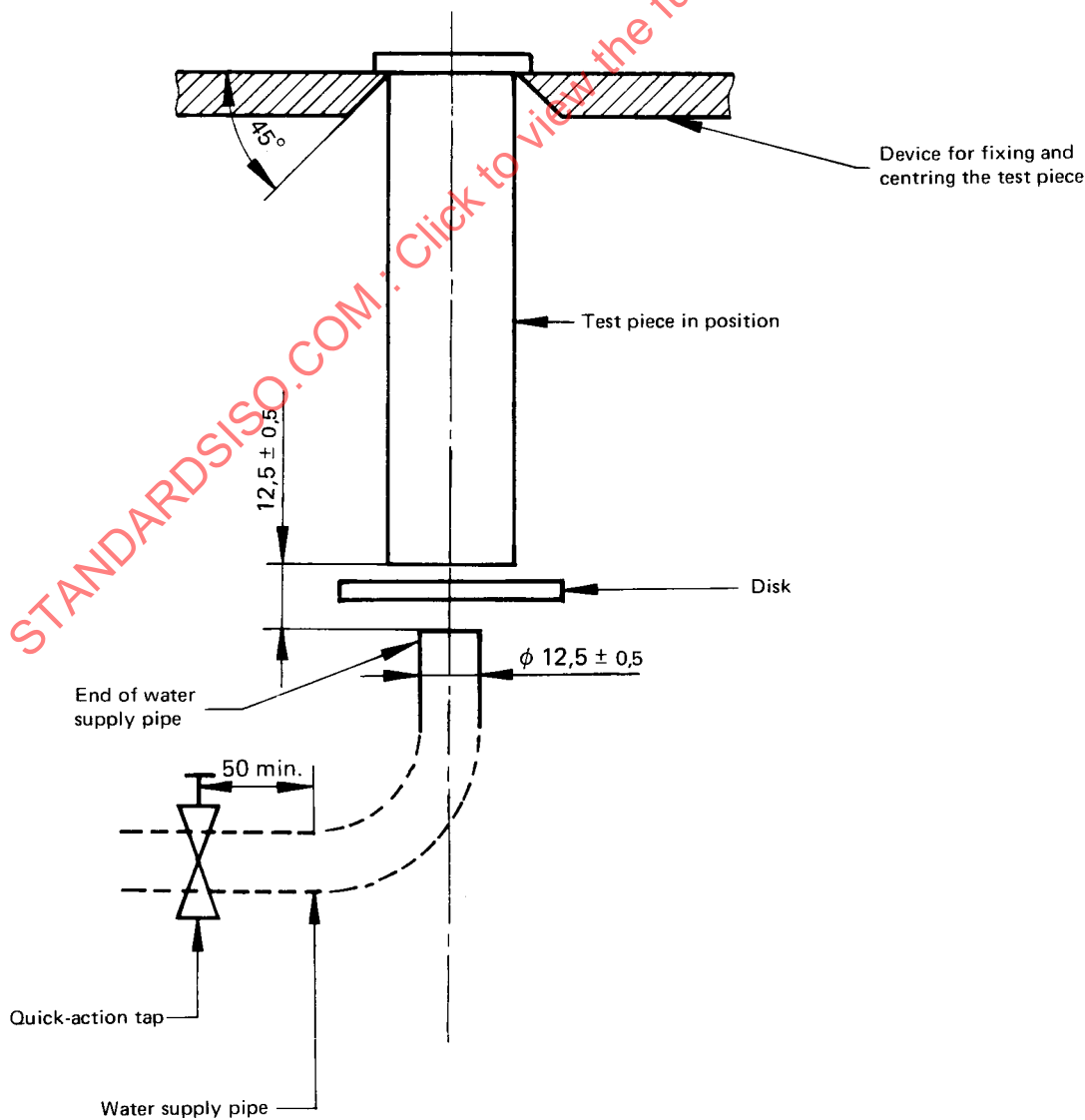
FIGURE 4 – Diagram of quenching device
