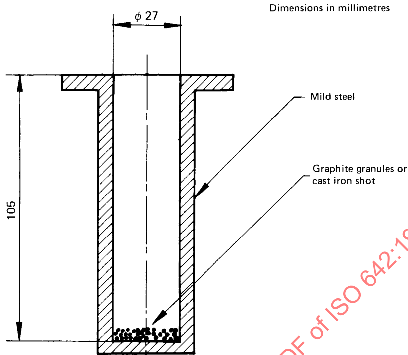
FIGURE 3 – Example of a mild steel vessel for heating the test piece
