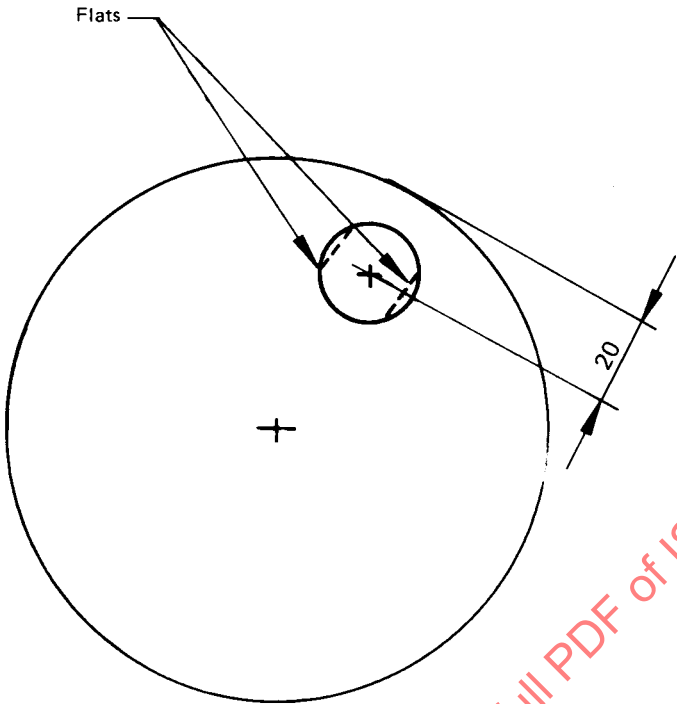
FIGURE 1 – Sampling by machining of the test piece
