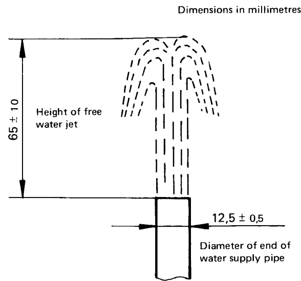
FIGURE 5 — End of water supply pipe
