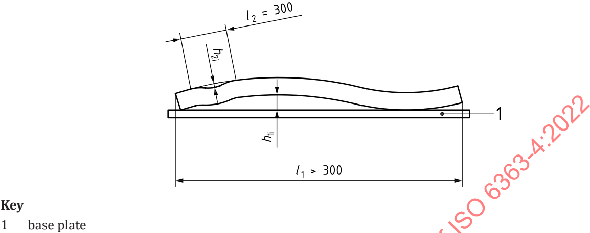
Figure 2 — Measurement of deviation from straightness
