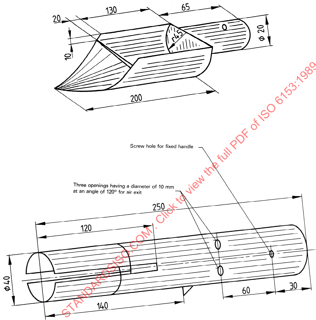
Figure 3 — Increment probes
