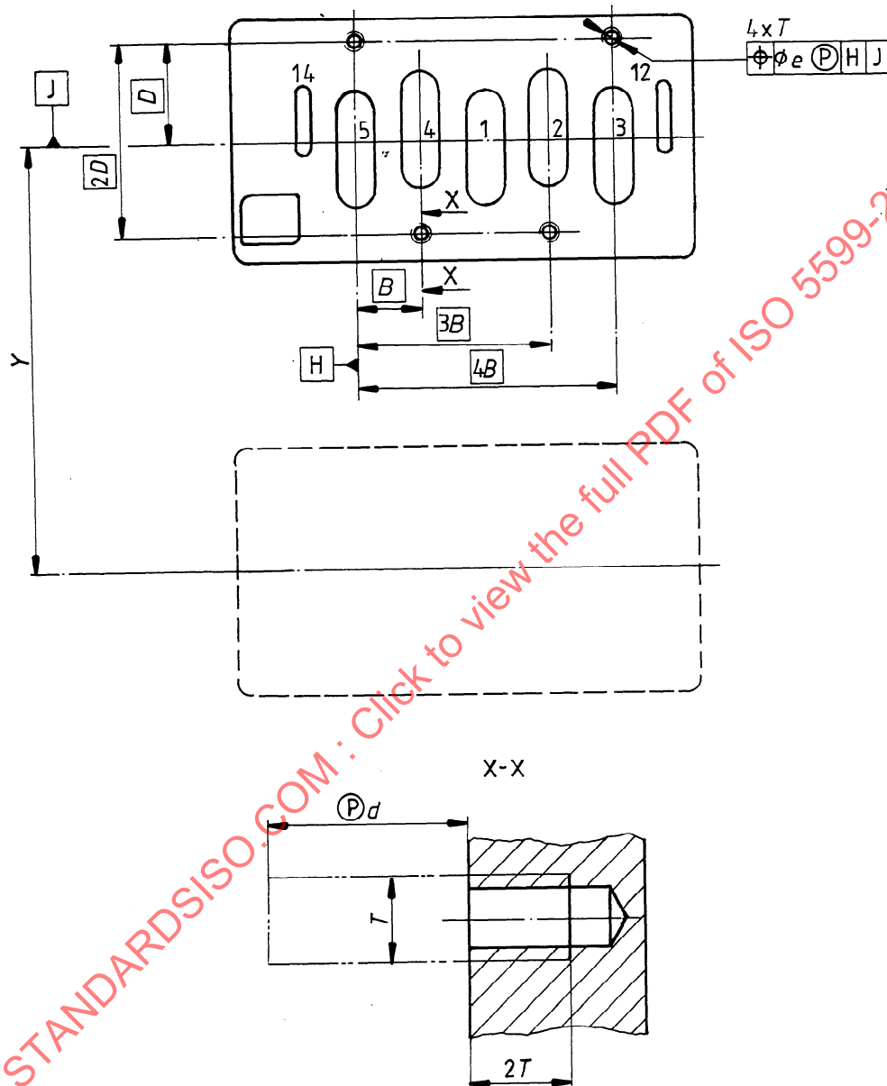
Figure 4 — Identification of main and actuation orifices and tolerances of position of the mounting surface — Sizes 1E, 2E and 3E
