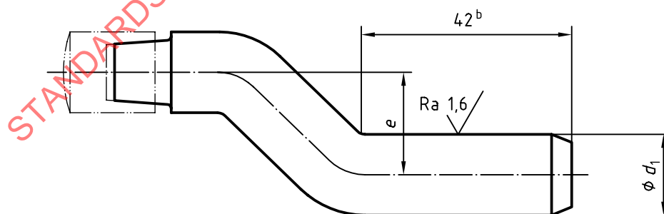
c) Type E: Double cranked adaptor
